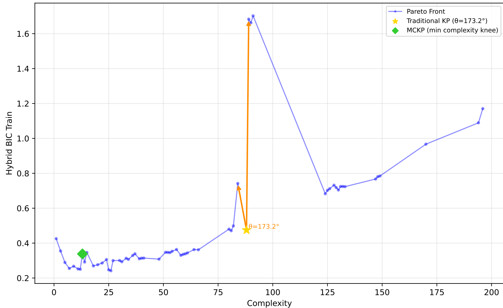
192_vineyard - Run 6 - MVP - Hybrid BIC Train \lambda_1=0.00, \lambda_2=0.30, \lambda_3=1.00 | Difficulty: 1.00 | Method: hmr
