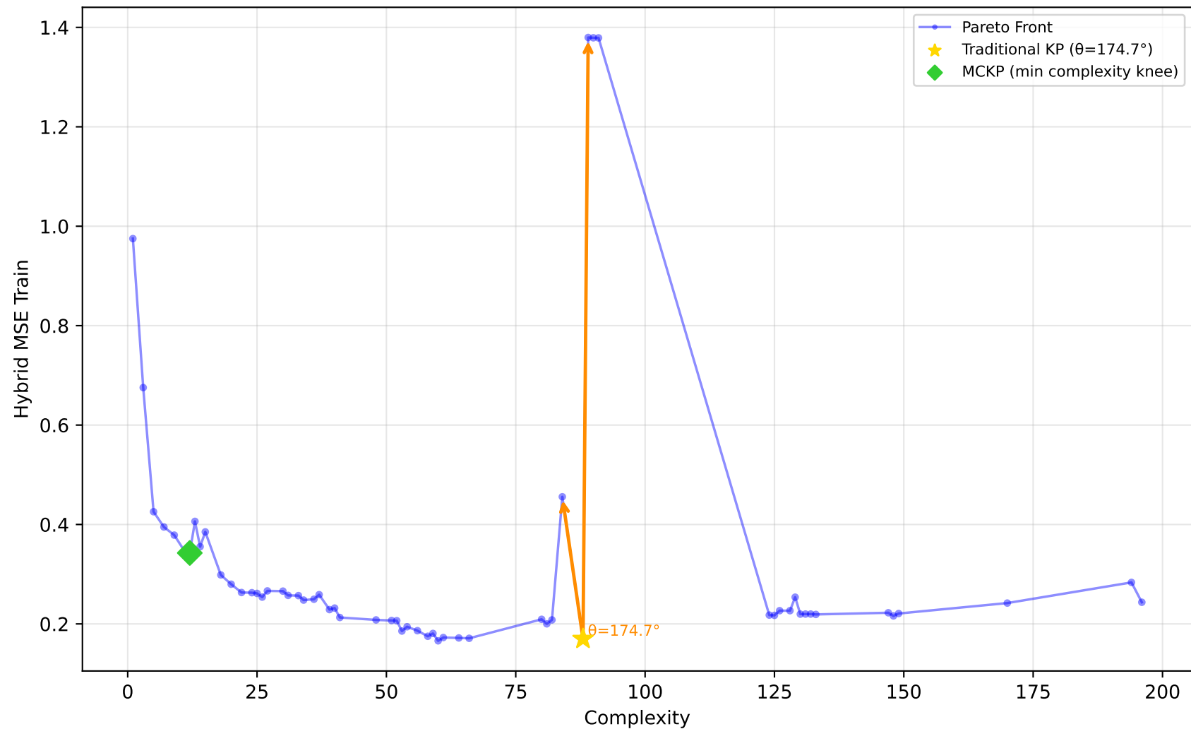
192_vineyard - Run 6 - MVP - Hybrid MSE Train \lambda_1=0.00, \bar{\lambda}_2=0.30, \lambda_3=1.00 | Difficulty: 1.00 | Method: hmr
