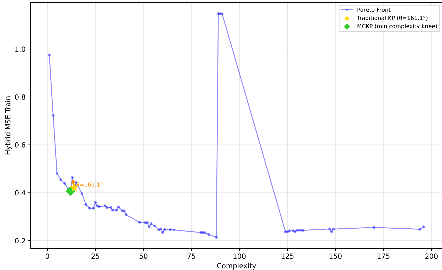
192_vineyard - Run 6 - MVP - Hybrid MSE Train \lambda_1=0.40, \bar{\lambda}_2=0.00, \lambda_3=1.00 | Difficulty: 1.00 | Method: hmr
