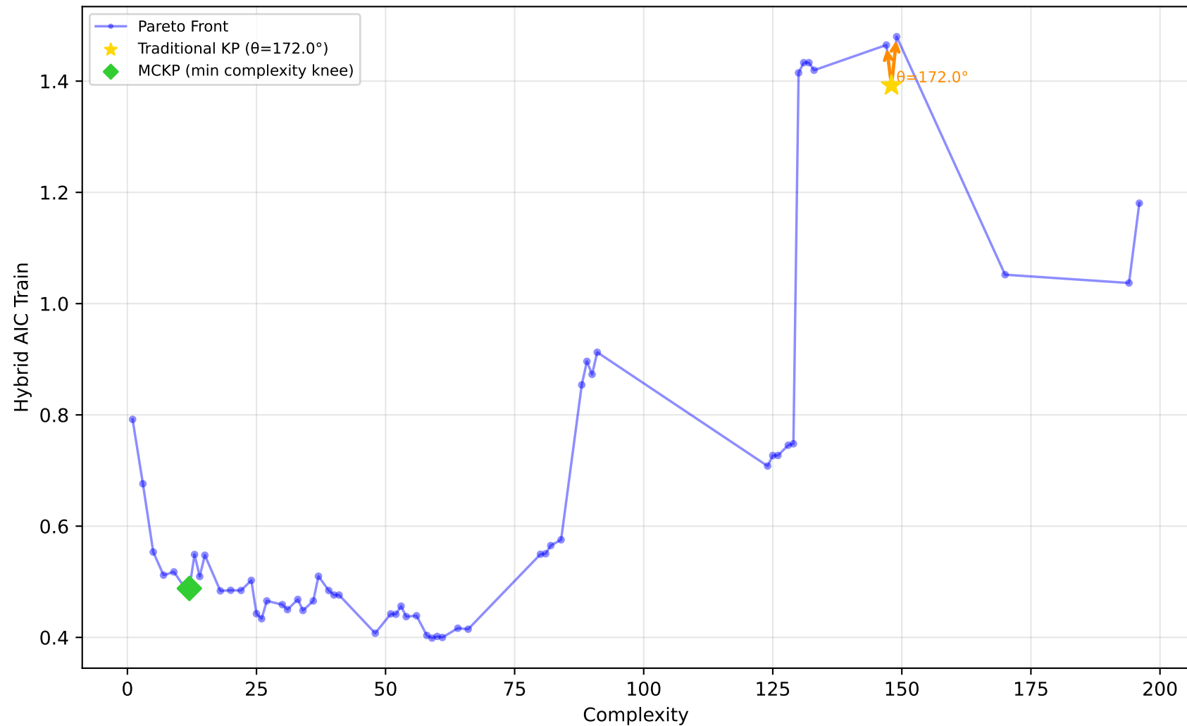
192_vineyard - Run 6 - SVP - Hybrid AIC Train \lambda_1=0.00, \lambda_2=1.00, \lambda_3=1.00 | Difficulty: 1.00 | Method: hmr
