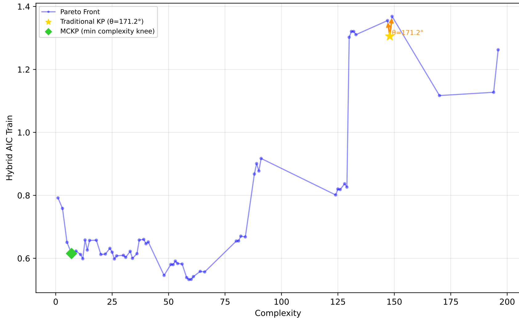
192_vineyard - Run 6 - SVP - Hybrid AIC Train \lambda_1=0.70, \lambda_2=0.70, \lambda_3=0.90 | Difficulty: 1.00 | Method: hmr
