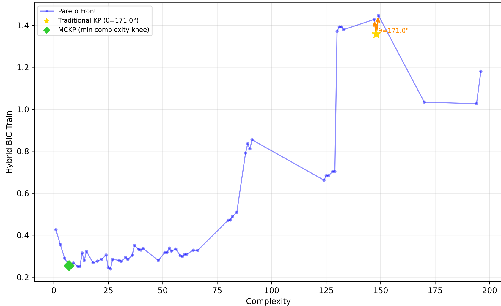
192_vineyard - Run 6 - SVP - Hybrid BIC Train \lambda_1=0.00, \lambda_2=1.00, \lambda_3=1.00 | Difficulty: 1.00 | Method: hmr
