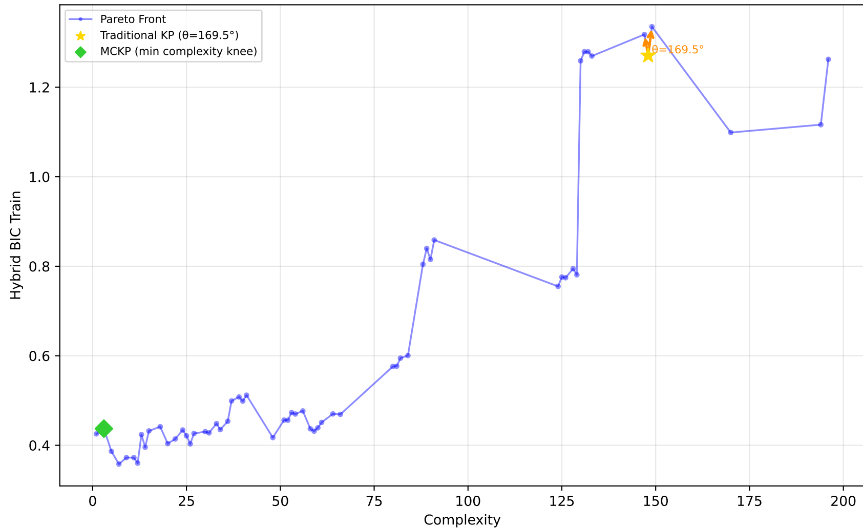
192_vineyard - Run 6 - SVP - Hybrid BIC Train \lambda_1=0.70, \lambda_2=0.70, \lambda_3=0.90 | Difficulty: 1.00 | Method: hmr
