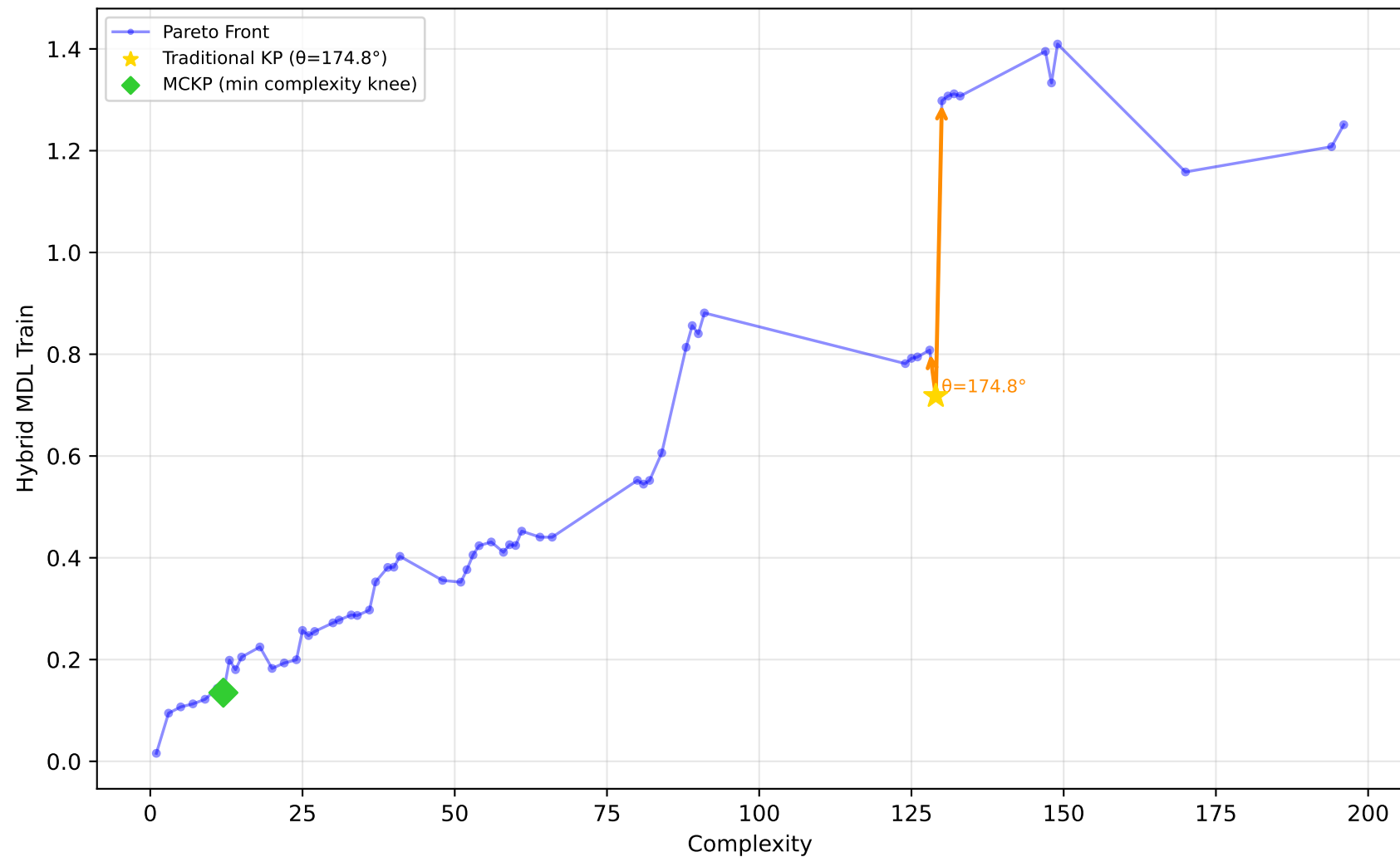
192_vineyard - Run 6 - SVP - Hybrid MDL Train \lambda_1=0.70, \bar{\lambda}_2=0.70, \lambda_3=0.90 | Difficulty: 1.00 | Method: hmr
