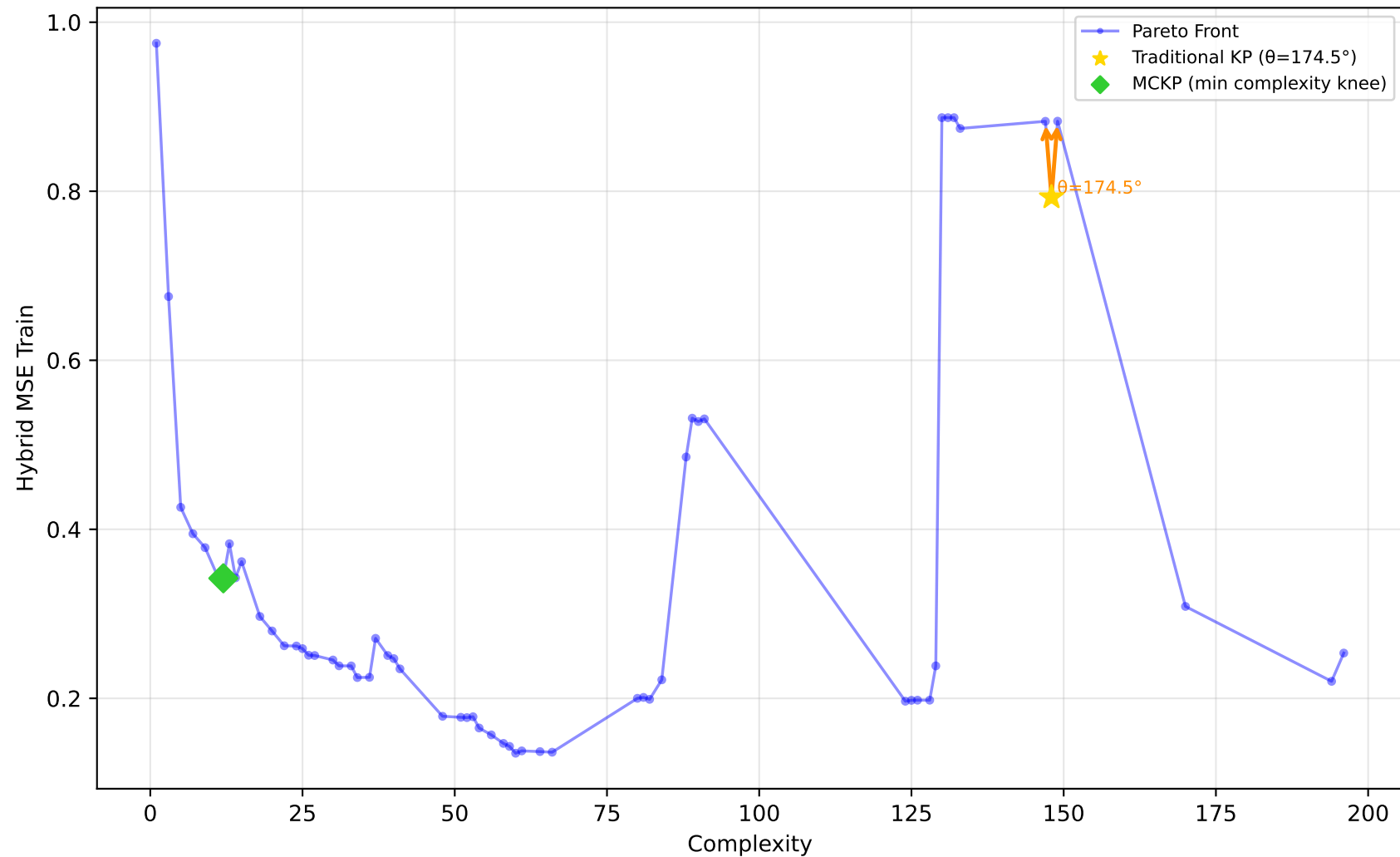
192_vineyard - Run 6 - SVP - Hybrid MSE Train \lambda_1=0.00, \lambda_2=1.00, \lambda_3=1.00 | Difficulty: 1.00 | Method: hmr
