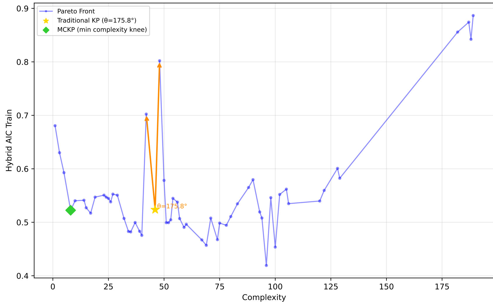
192_vineyard - Run 7 - MVP - Hybrid AIC Train \lambda_1=0.40, \lambda_2=0.00, \lambda_3=1.00 | Difficulty: 1.00 | Method: hmr
