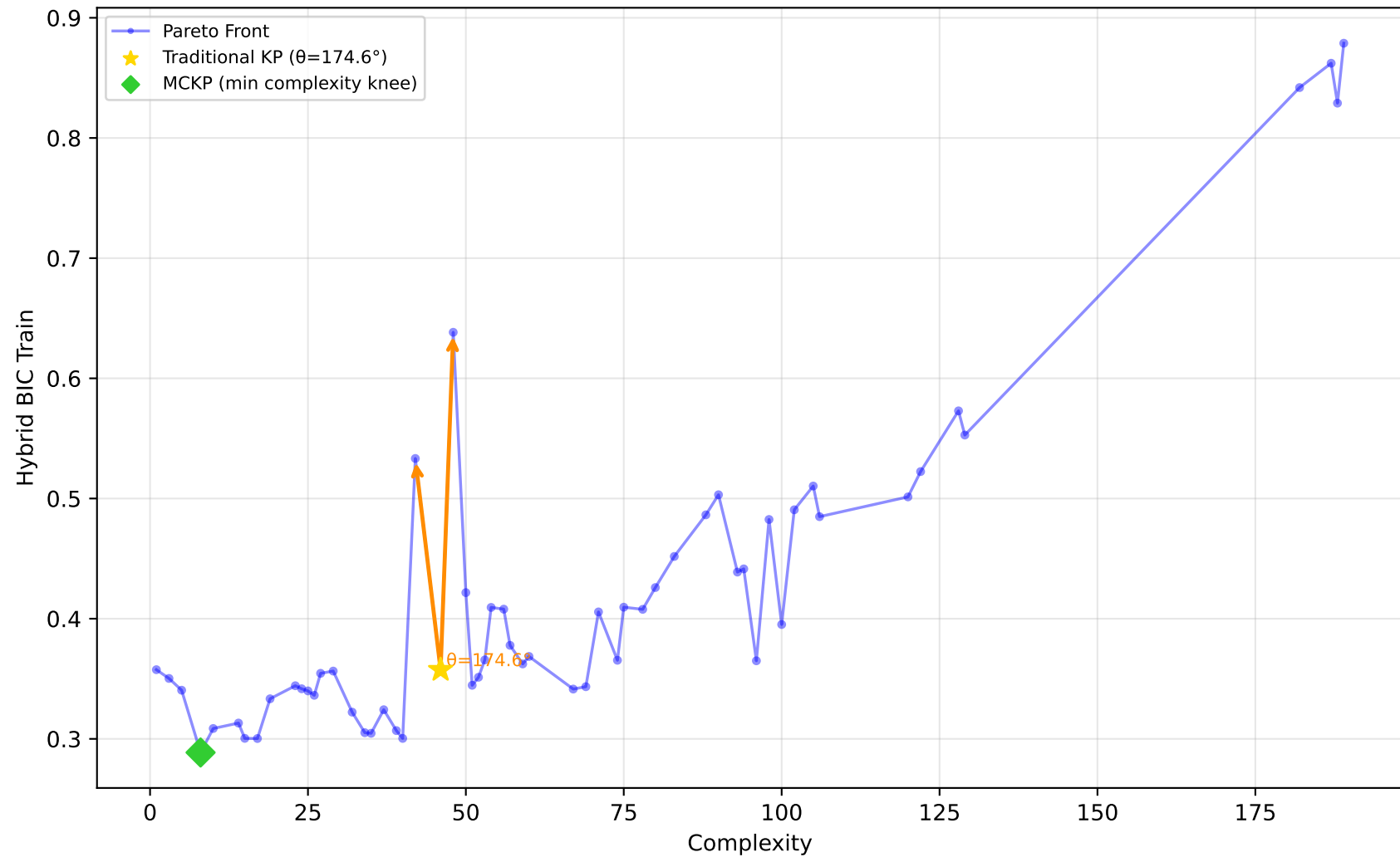
192_vineyard - Run 7 - MVP - Hybrid BIC Train \lambda_1=0.40, \lambda_2=0.00, \lambda_3=1.00 | Difficulty: 1.00 | Method: hmr
