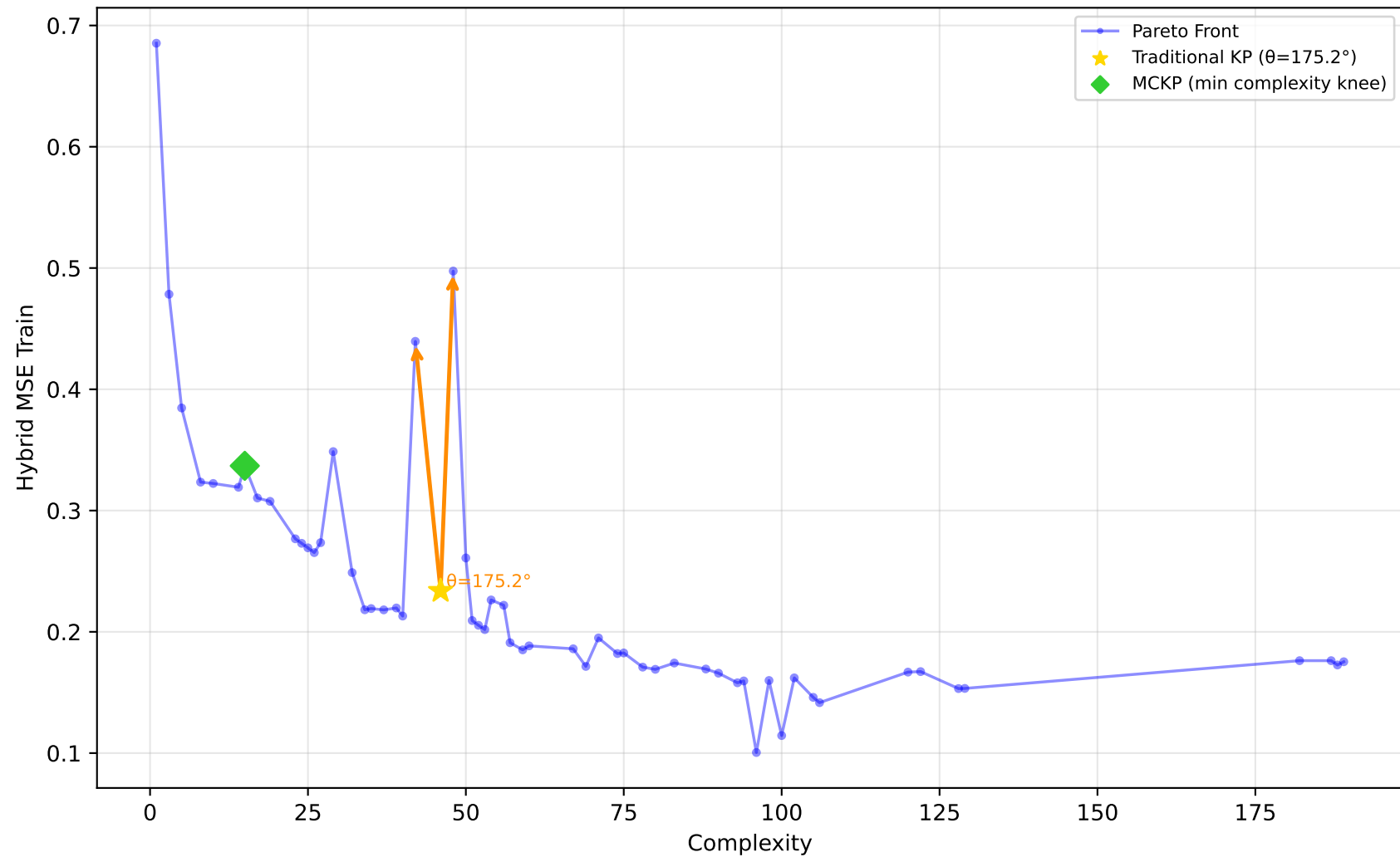
192_vineyard - Run 7 - MVP - Hybrid MSE Train \lambda_1=0.00, \bar{\lambda}_2=0.30, \lambda_3=1.00 | Difficulty: 1.00 | Method: hmr
