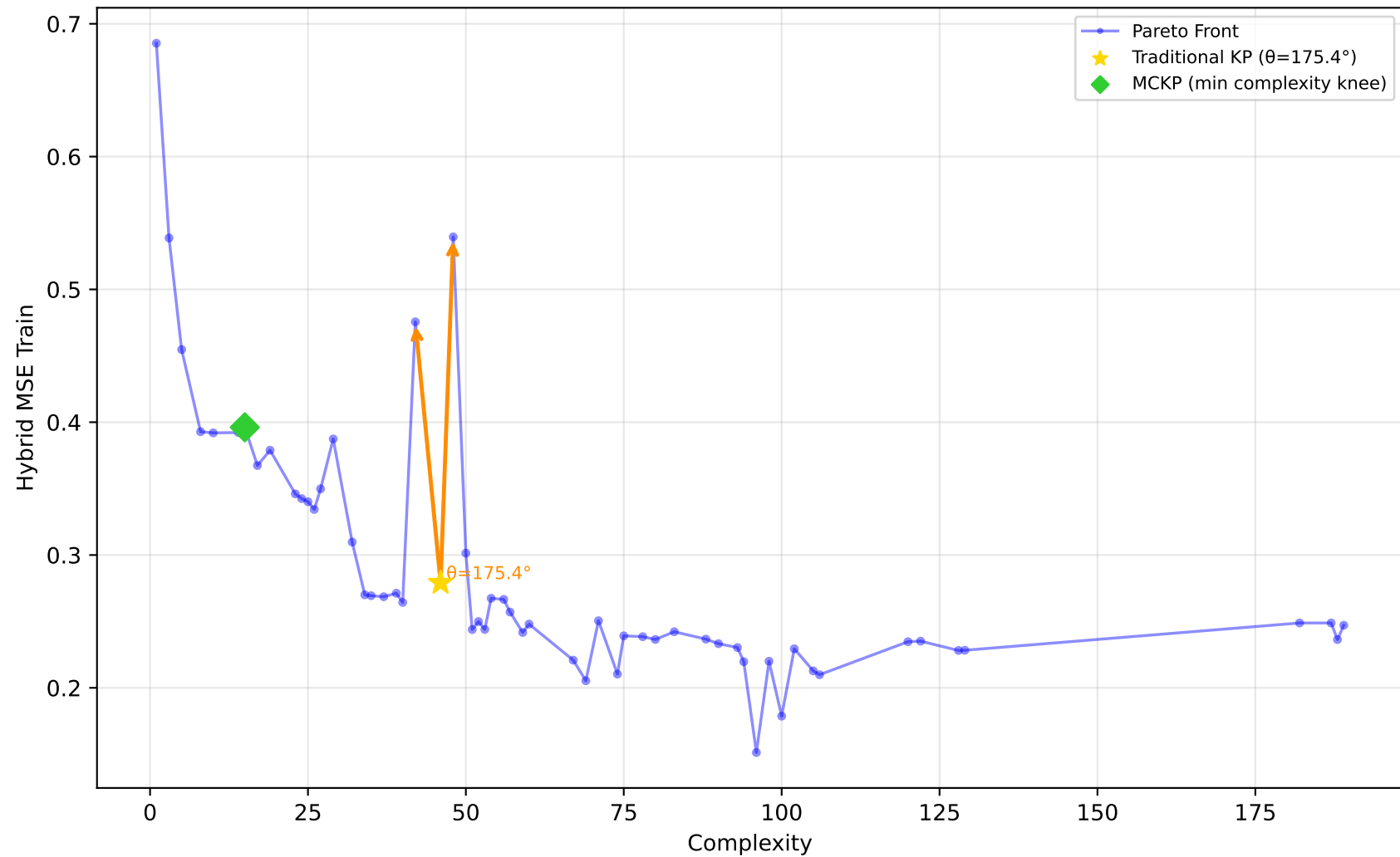
192_vineyard - Run 7 - MVP - Hybrid MSE Train \lambda_1=0.40, \bar{\lambda}_2=0.00, \lambda_3=1.00 | Difficulty: 1.00 | Method: hmr
