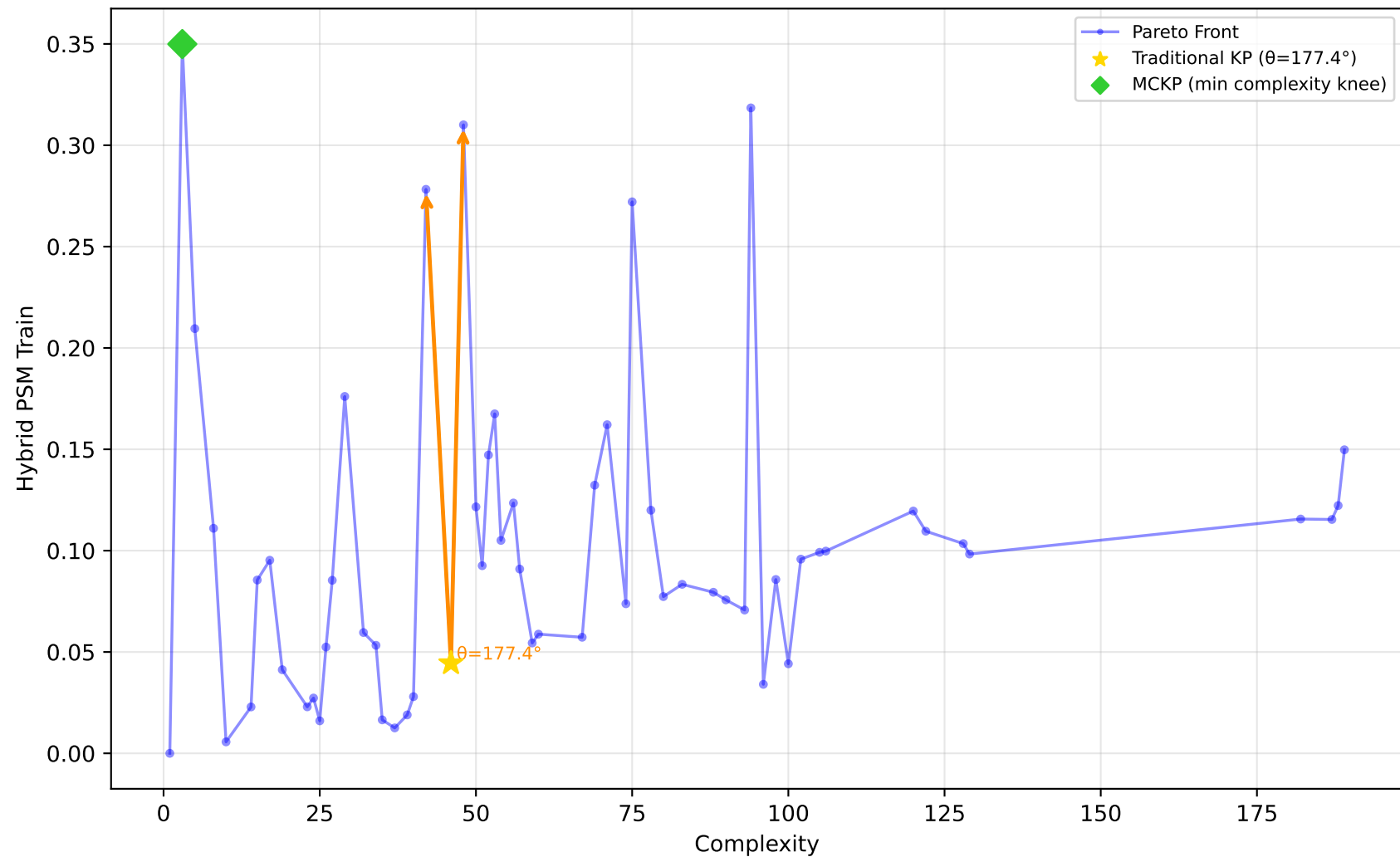
192_vineyard - Run 7 - MVP - Hybrid PSM Train \lambda_1=0.00 , \lambda_2=0.30 , \lambda_3=1.00 | Difficulty: 1.00 | Method: hmr
