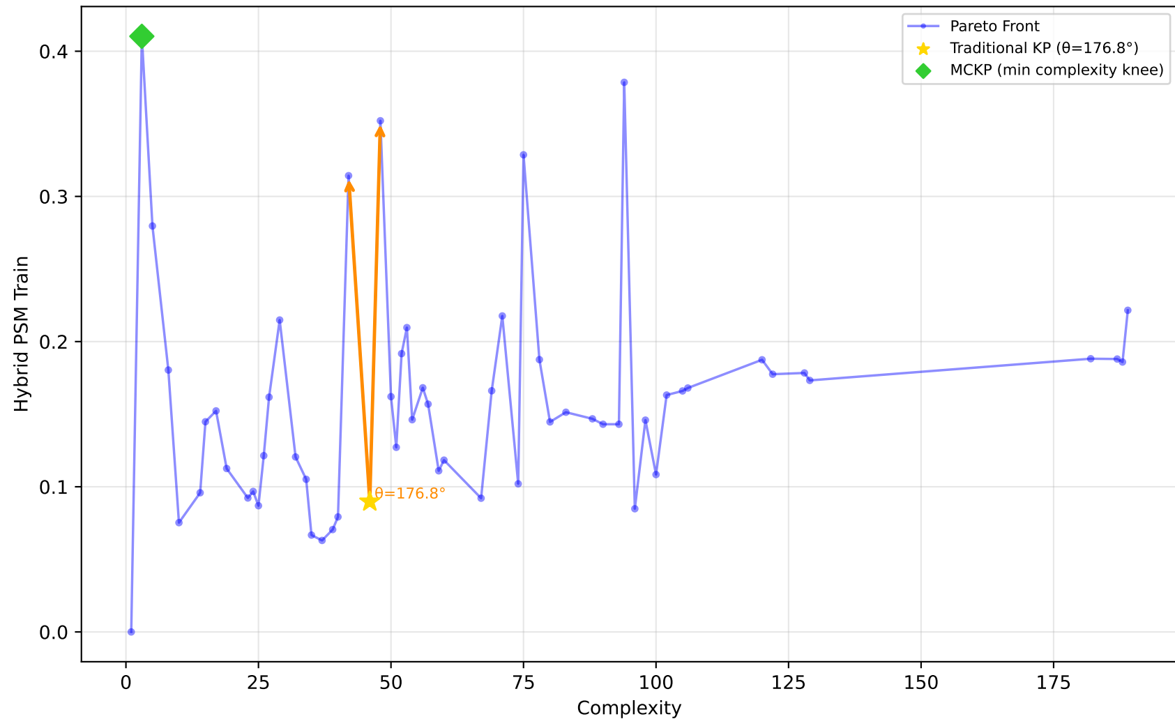
192_vineyard - Run 7 - MVP - Hybrid PSM Train \lambda_1=0.40, \bar{\lambda}_2=0.00, \lambda_3=1.00 | Difficulty: 1.00 | Method: hmr
