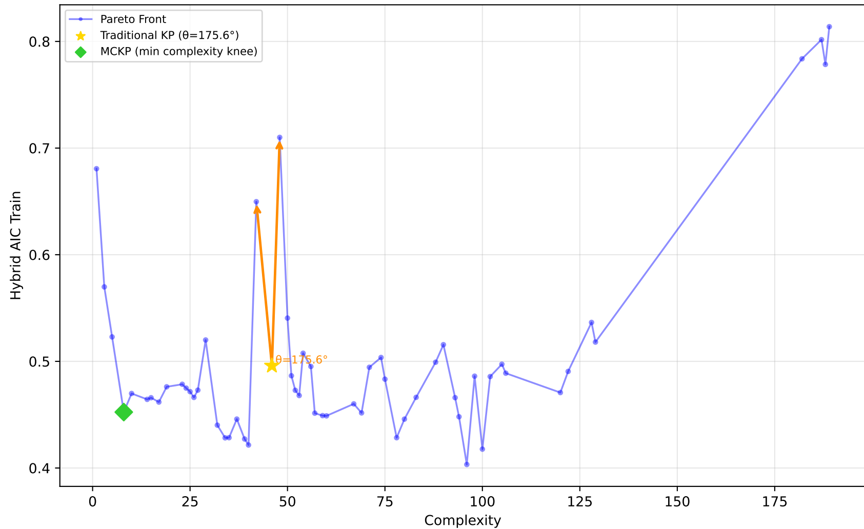
192_vineyard - Run 7 - SVP - Hybrid AIC Train \lambda_1=0.00, \lambda_2=1.00, \lambda_3=1.00 | Difficulty: 1.00 | Method: hmr
