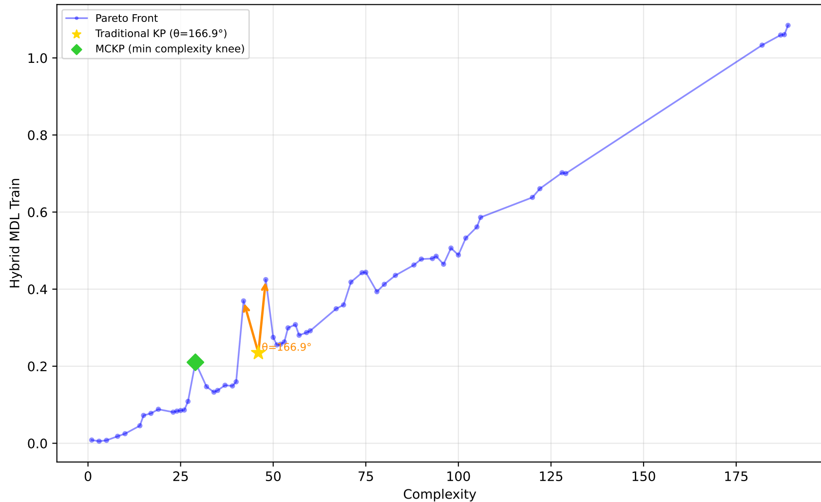
192_vineyard - Run 7 - SVP - Hybrid MDL Train \lambda_1=0.00, \bar{\lambda}_2=1.00, \lambda_3=1.00 | Difficulty: 1.00 | Method: hmr
