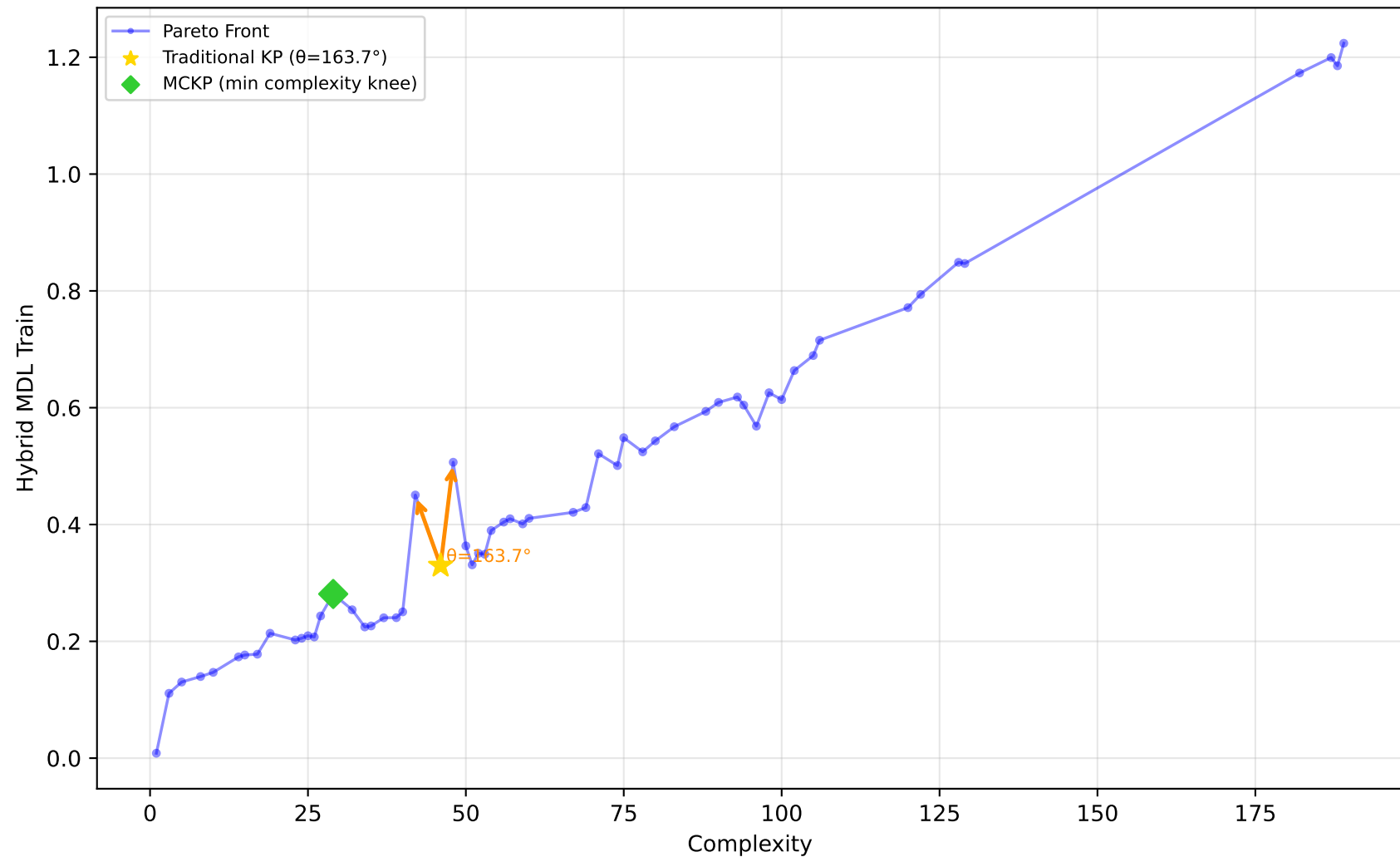
192_vineyard - Run 7 - SVP - Hybrid MDL Train \lambda_1=0.70, \lambda_2=0.70, \lambda_3=0.90 | Difficulty: 1.00 | Method: hmr
