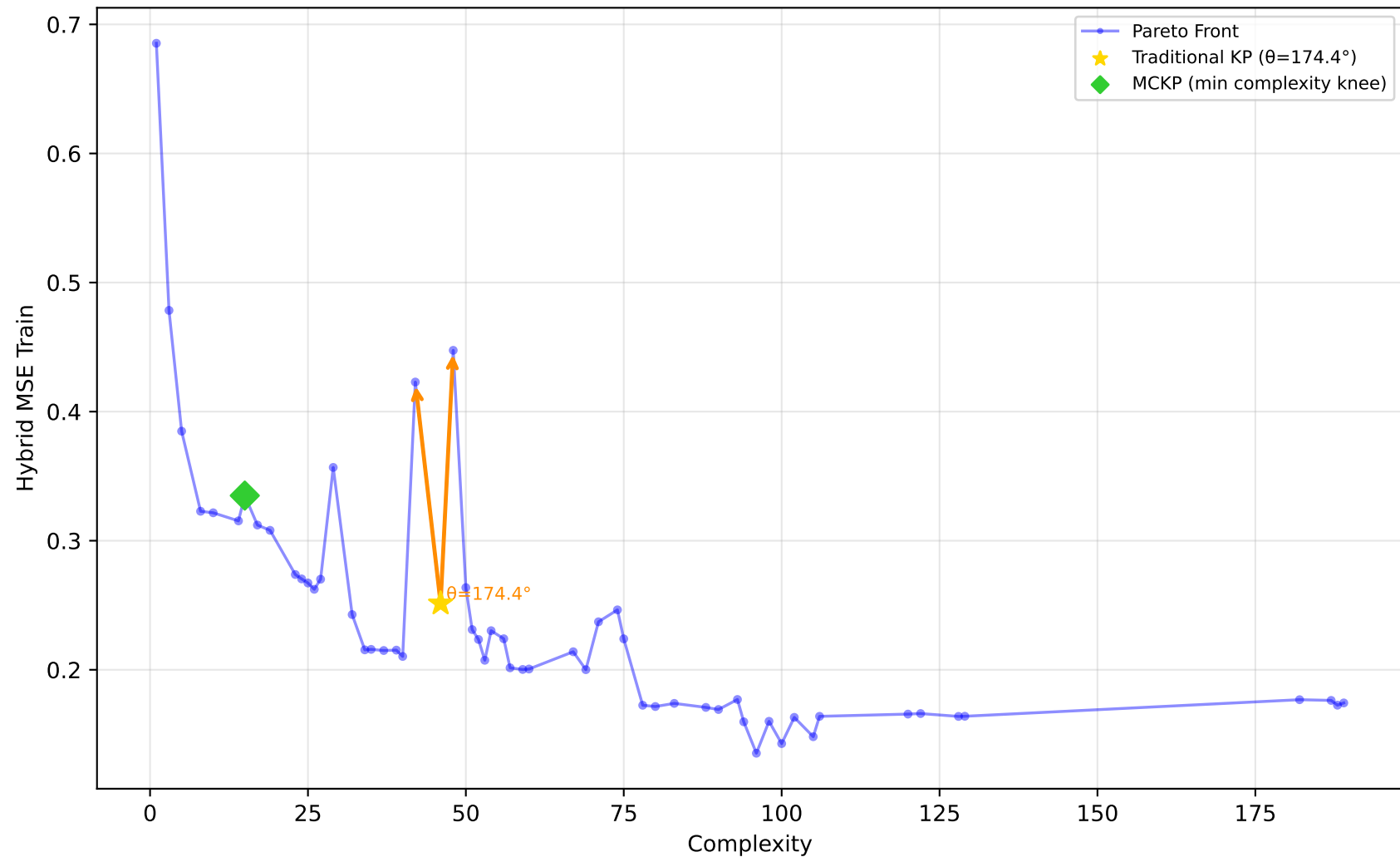
192_vineyard - Run 7 - SVP - Hybrid MSE Train \lambda_1=0.00, \bar{\lambda}_2=1.00, \lambda_3=1.00 | Difficulty: 1.00 | Method: hmr
