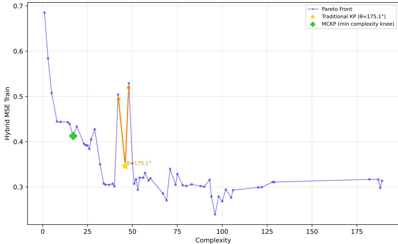
192_vineyard - Run 7 - SVP - Hybrid MSE Train \lambda_1=0.70, \lambda_2=0.70, \lambda_3=0.90 | Difficulty: 1.00 | Method: hmr
