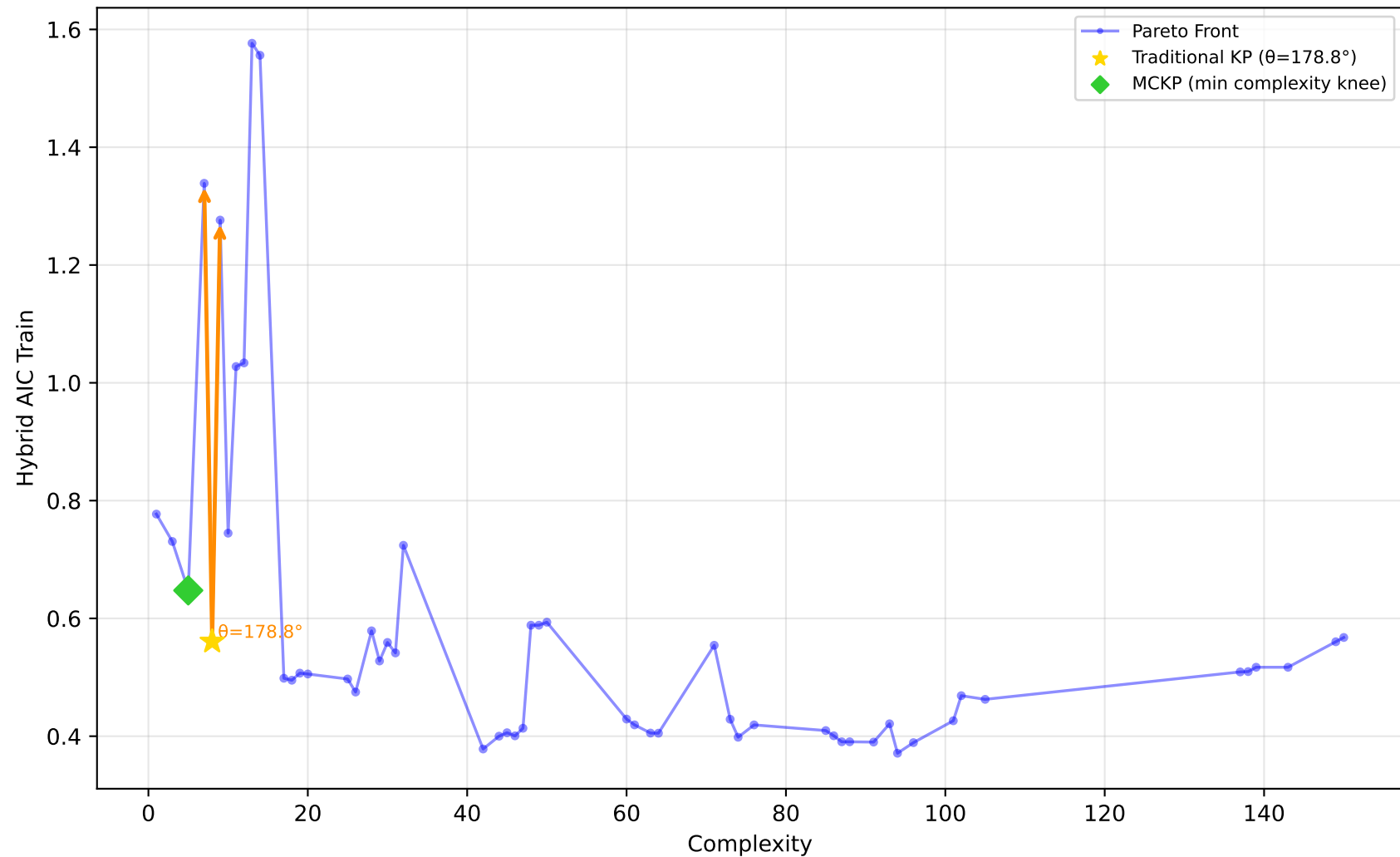
192_vineyard - Run 8 - MVP - Hybrid AIC Train \lambda_1=0.40, \lambda_2=0.00, \lambda_3=1.00 | Difficulty: 1.00 | Method: hmr
