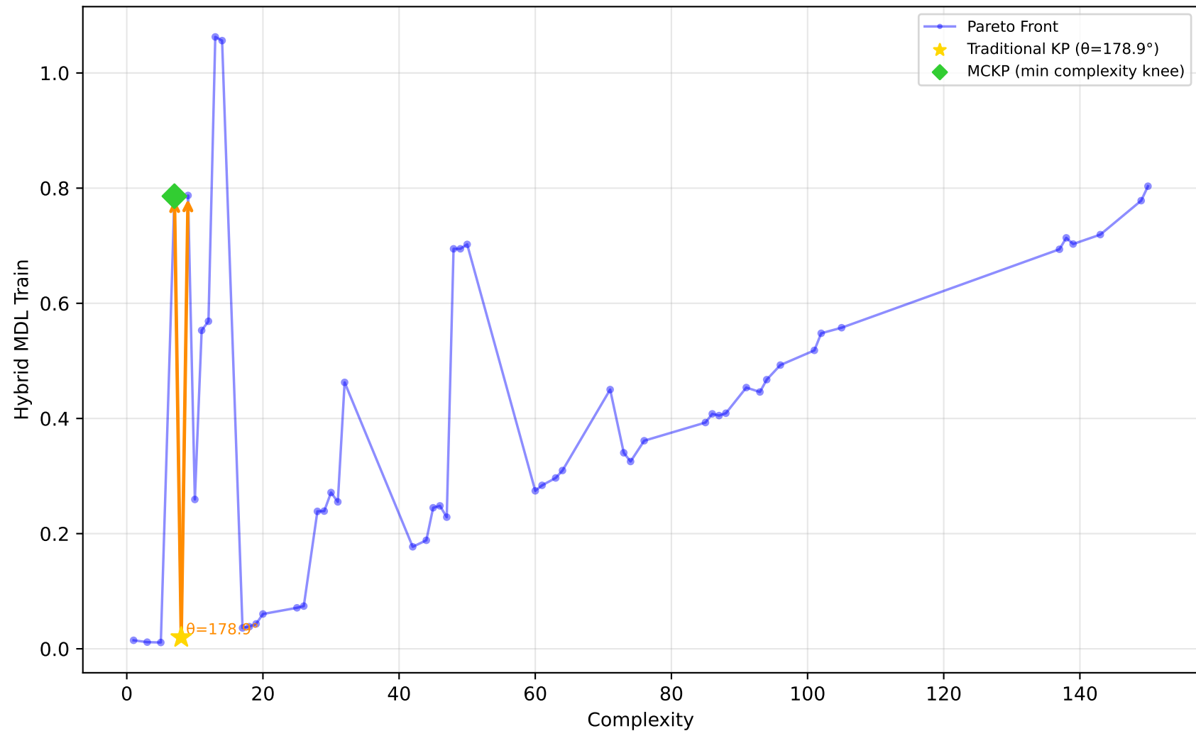
192_vineyard - Run 8 - MVP - Hybrid MDL Train \lambda_1=0.00, \bar{\lambda}_2=0.30, \lambda_3=1.00 | Difficulty: 1.00 | Method: hmr
