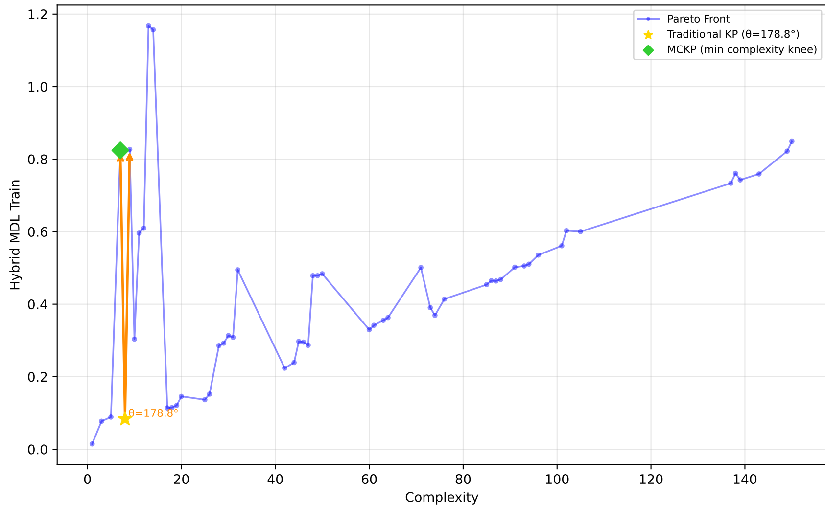
192_vineyard - Run 8 - MVP - Hybrid MDL Train \lambda_1=0.40, \bar{\lambda}_2=0.00, \lambda_3=1.00 | Difficulty: 1.00 | Method: hmr
