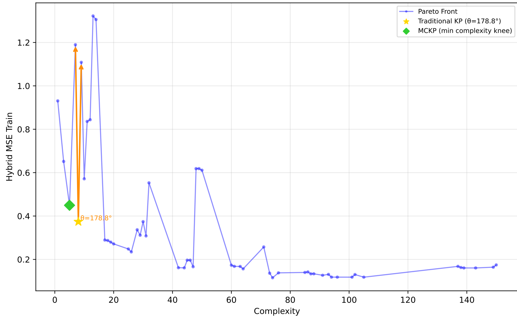
192_vineyard - Run 8 - MVP - Hybrid MSE Train \lambda_1=0.00, \bar{\lambda}_2=0.30, \lambda_3=1.00 | Difficulty: 1.00 | Method: hmr
