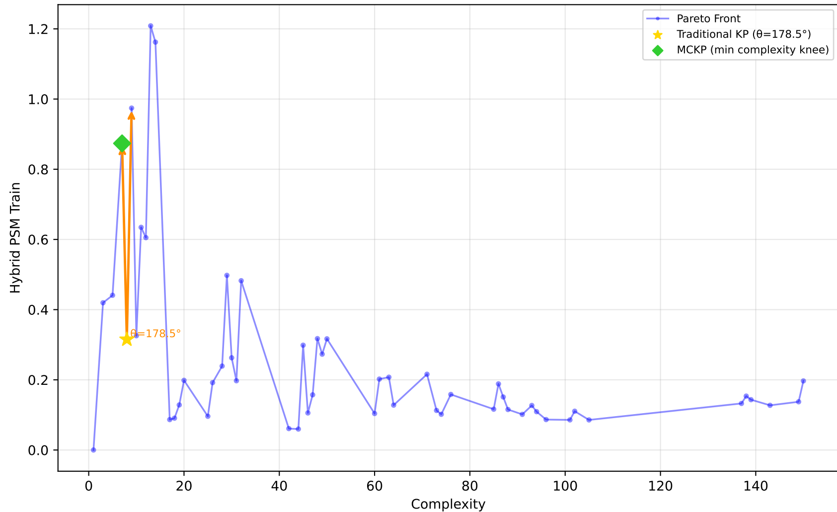
192_vineyard - Run 8 - MVP - Hybrid PSM Train \lambda_1=0.40, \bar{\lambda}_2=0.00, \lambda_3=1.00 | Difficulty: 1.00 | Method: hmr
