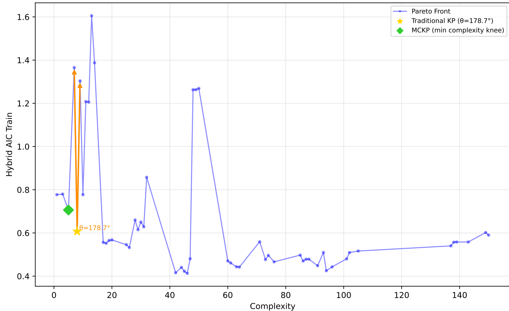
192_vineyard - Run 8 - SVP - Hybrid AIC Train \lambda_1=0.70, \lambda_2=0.70, \lambda_3=0.90 | Difficulty: 1.00 | Method: hmr
