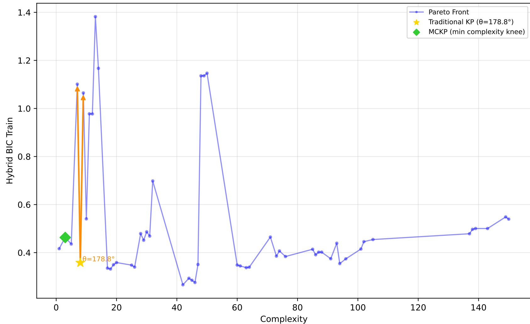
192_vineyard - Run 8 - SVP - Hybrid BIC Train \lambda_1=0.70, \lambda_2=0.70, \lambda_3=0.90 | Difficulty: 1.00 | Method: hmr
