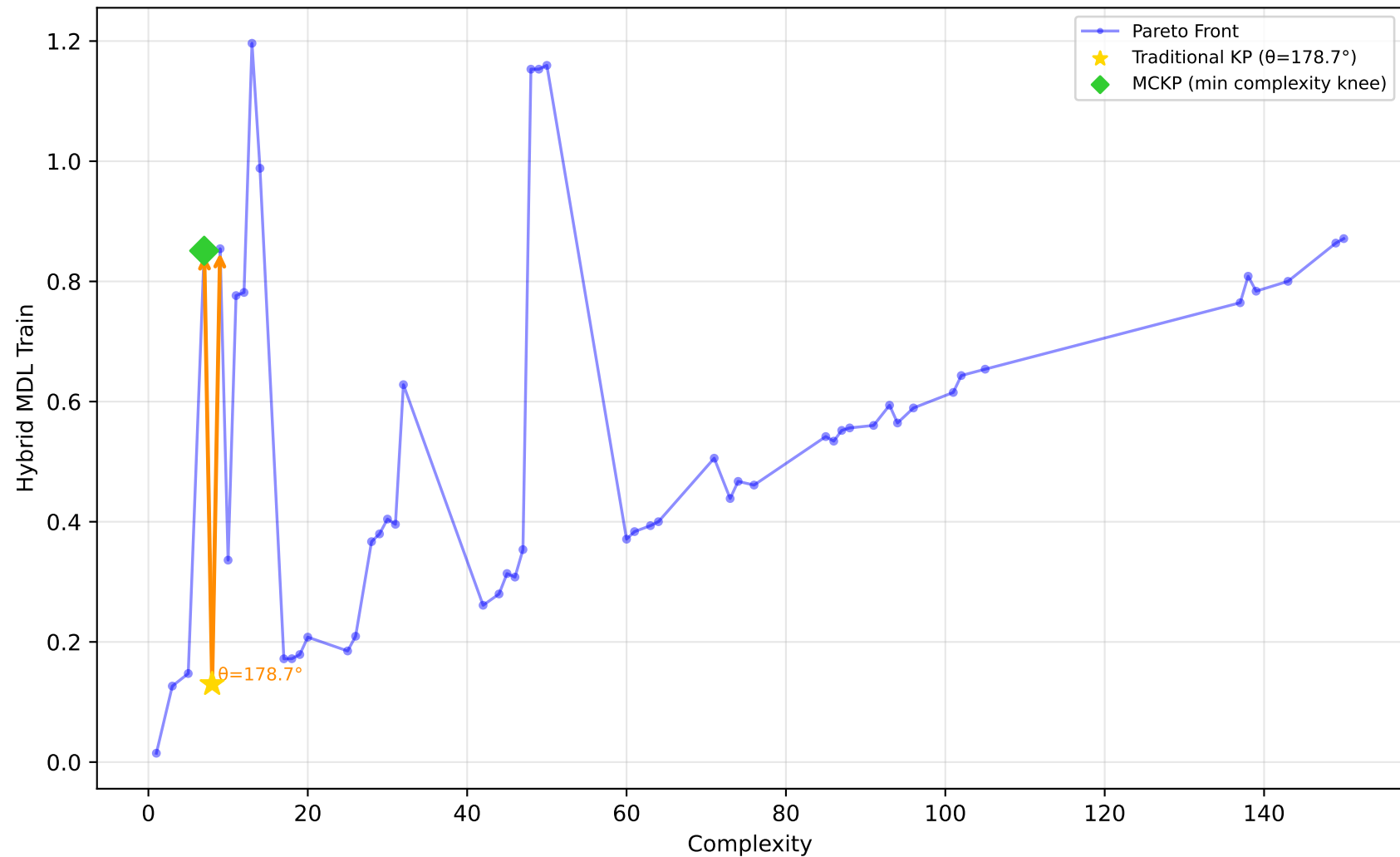
192_vineyard - Run 8 - SVP - Hybrid MDL Train \lambda_1=0.70, \bar{\lambda}_2=0.70, \lambda_3=0.90 | Difficulty: 1.00 | Method: hmr
