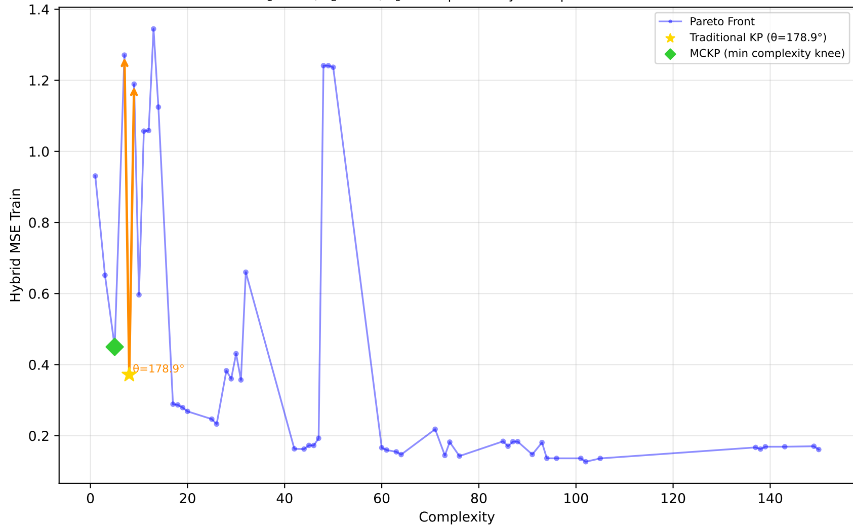
192_vineyard - Run 8 - SVP - Hybrid MSE Train \lambda_1=0.00, \bar{\lambda}_2=1.00, \lambda_3=1.00 | Difficulty: 1.00 | Method: hmr
