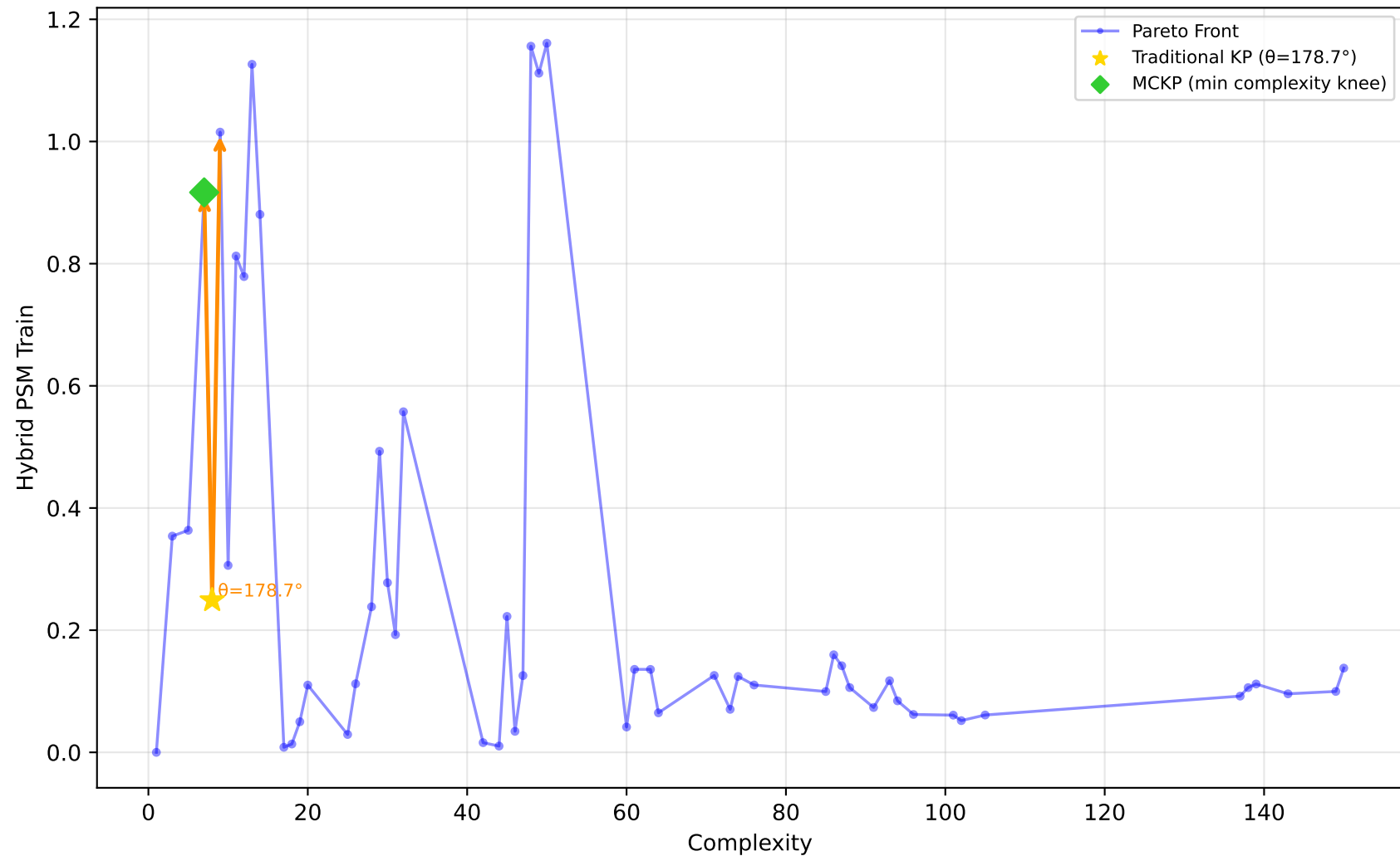
192_vineyard - Run 8 - SVP - Hybrid PSM Train \lambda_1=0.00, \bar{\lambda}_2=1.00, \lambda_3=1.00 | Difficulty: 1.00 | Method: hmr
