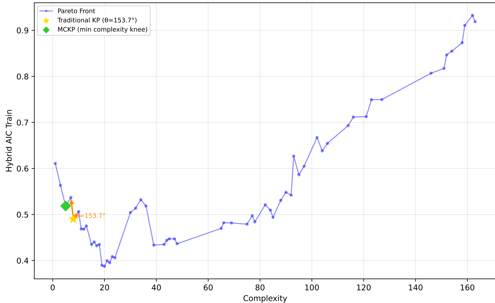
192_vineyard - Run 9 - MVP - Hybrid AIC Train \lambda_1=0.40, \lambda_2=0.00, \lambda_3=1.00 | Difficulty: 1.00 | Method: hmr
