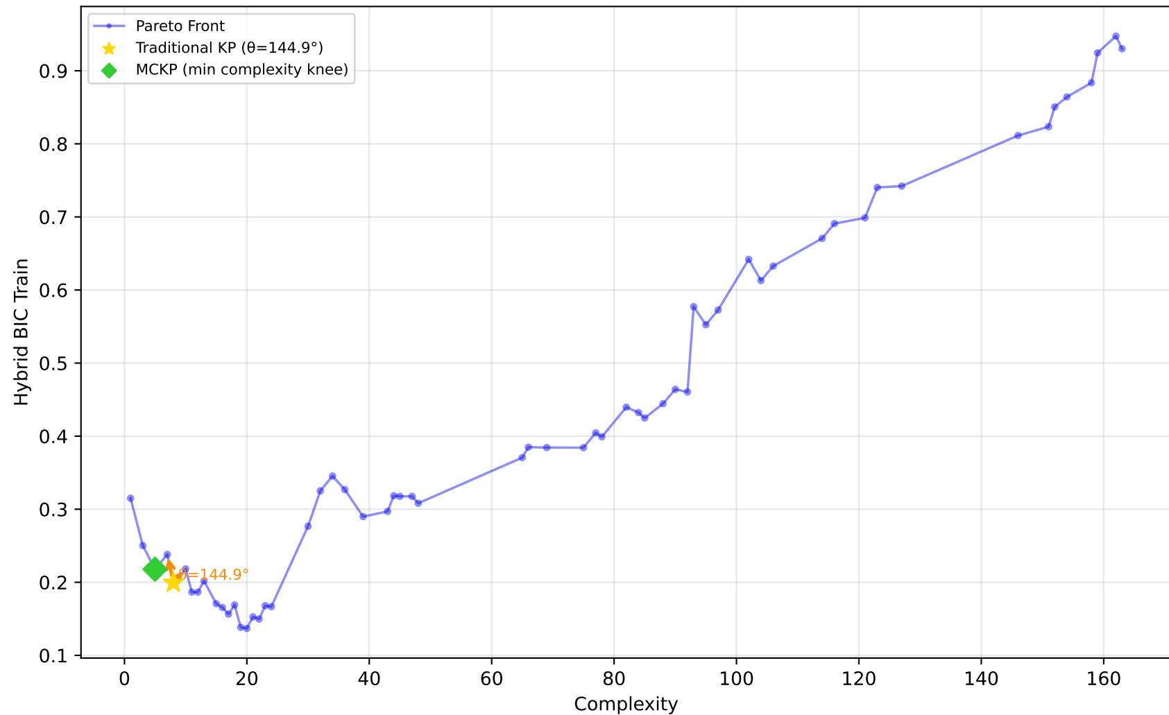
192_vineyard - Run 9 - MVP - Hybrid BIC Train \lambda_1=0.00, \lambda_2=0.30, \lambda_3=1.00 | Difficulty: 1.00 | Method: hmr
