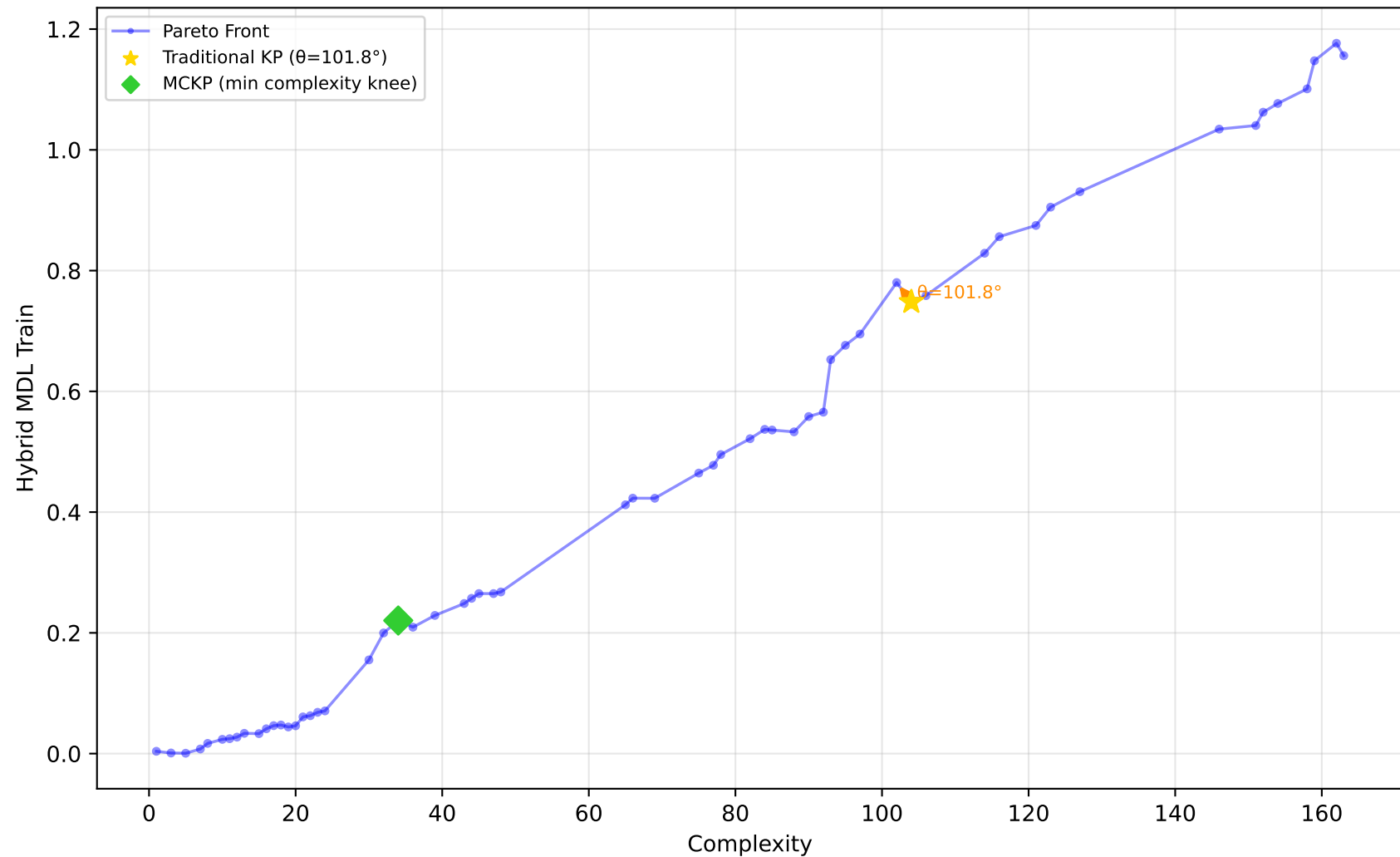
192_vineyard - Run 9 - MVP - Hybrid MDL Train \lambda_1=0.00, \bar{\lambda}_2=0.30, \lambda_3=1.00 | Difficulty: 1.00 | Method: hmr
