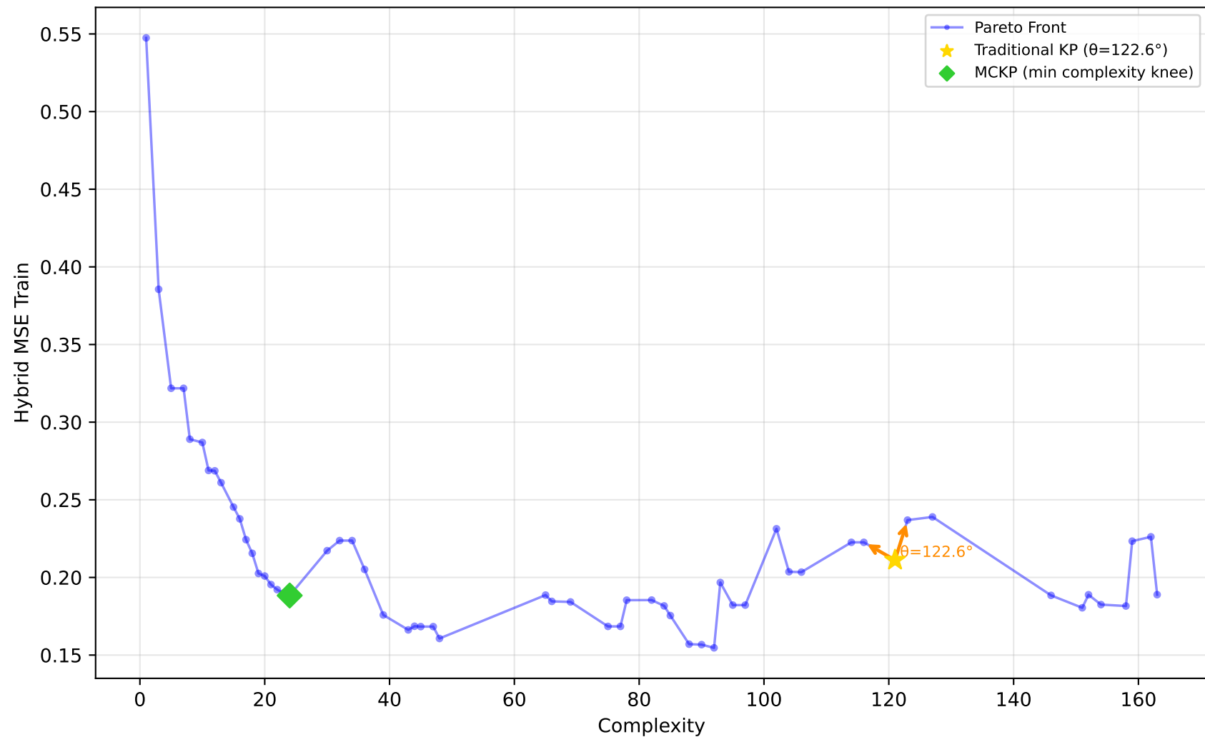
192_vineyard - Run 9 - MVP - Hybrid MSE Train \lambda_1=0.00 , \lambda_2=0.30 , \lambda_3=1.00 | Difficulty: 1.00 | Method: hmr
