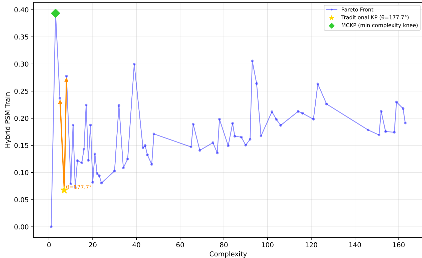
192_vineyard - Run 9 - MVP - Hybrid PSM Train \lambda_1=0.40, \bar{\lambda}_2=0.00, \lambda_3=1.00 | Difficulty: 1.00 | Method: hmr
