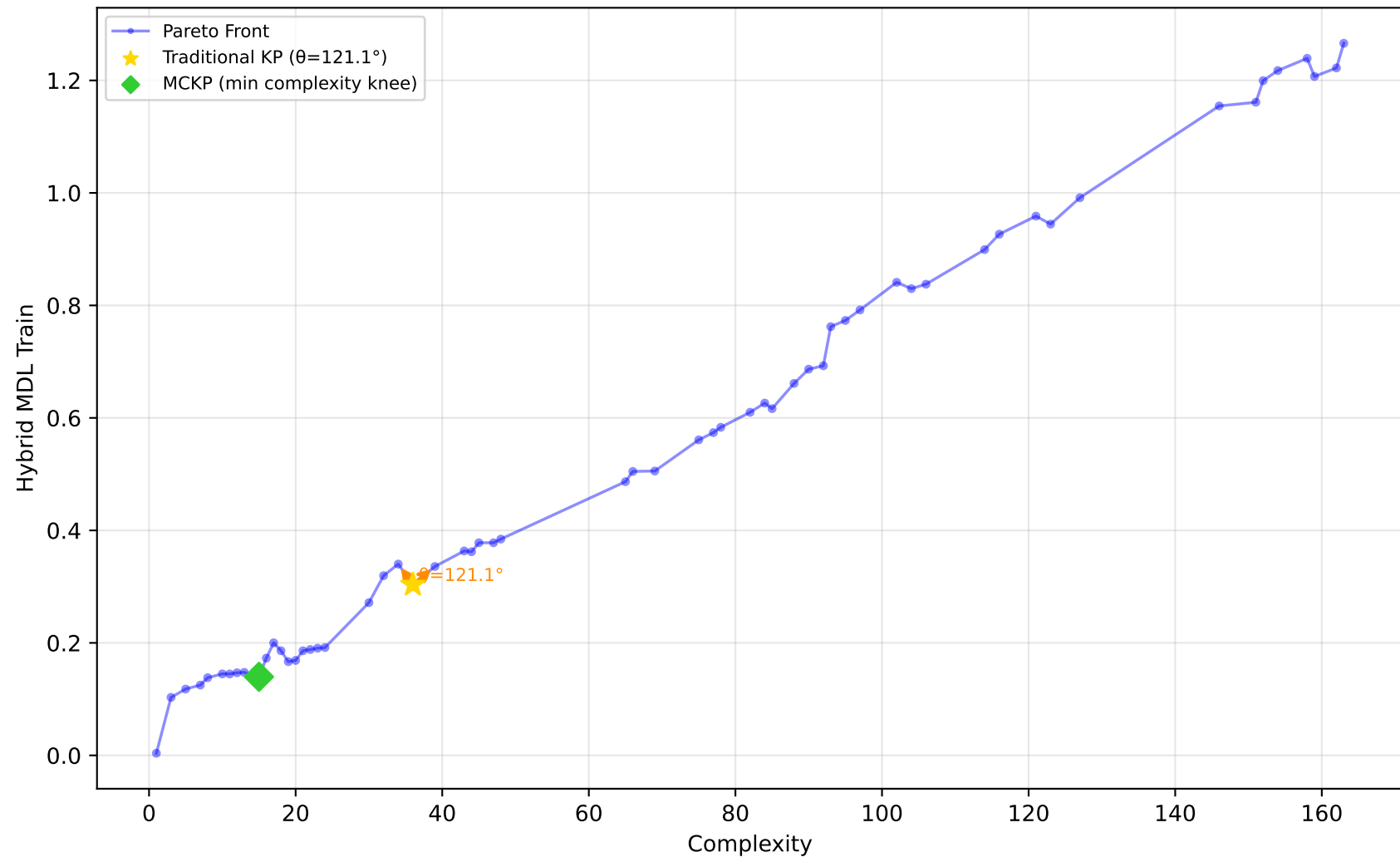
192_vineyard - Run 9 - SVP - Hybrid MDL Train \lambda_1=0.70, \bar{\lambda}_2=0.70, \lambda_3=0.90 | Difficulty: 1.00 | Method: hmr
