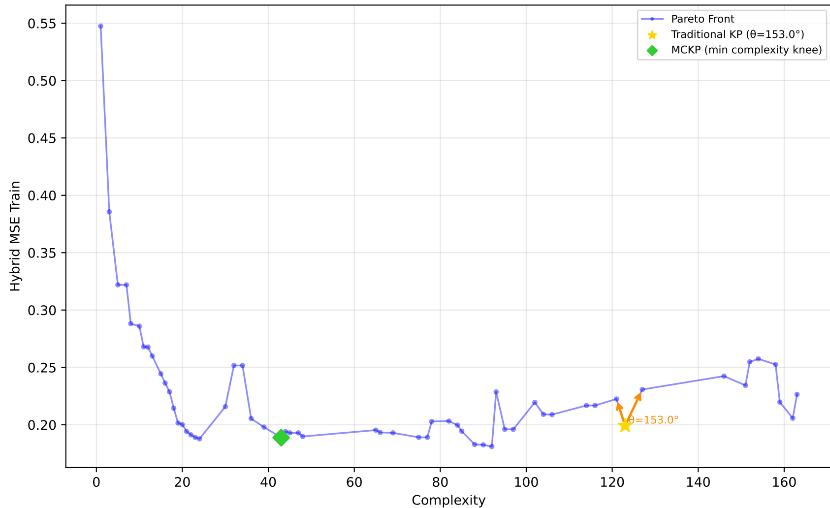
192_vineyard - Run 9 - SVP - Hybrid MSE Train \lambda_1=0.00, \lambda_2=1.00, \lambda_3=1.00 | Difficulty: 1.00 | Method: hmr
