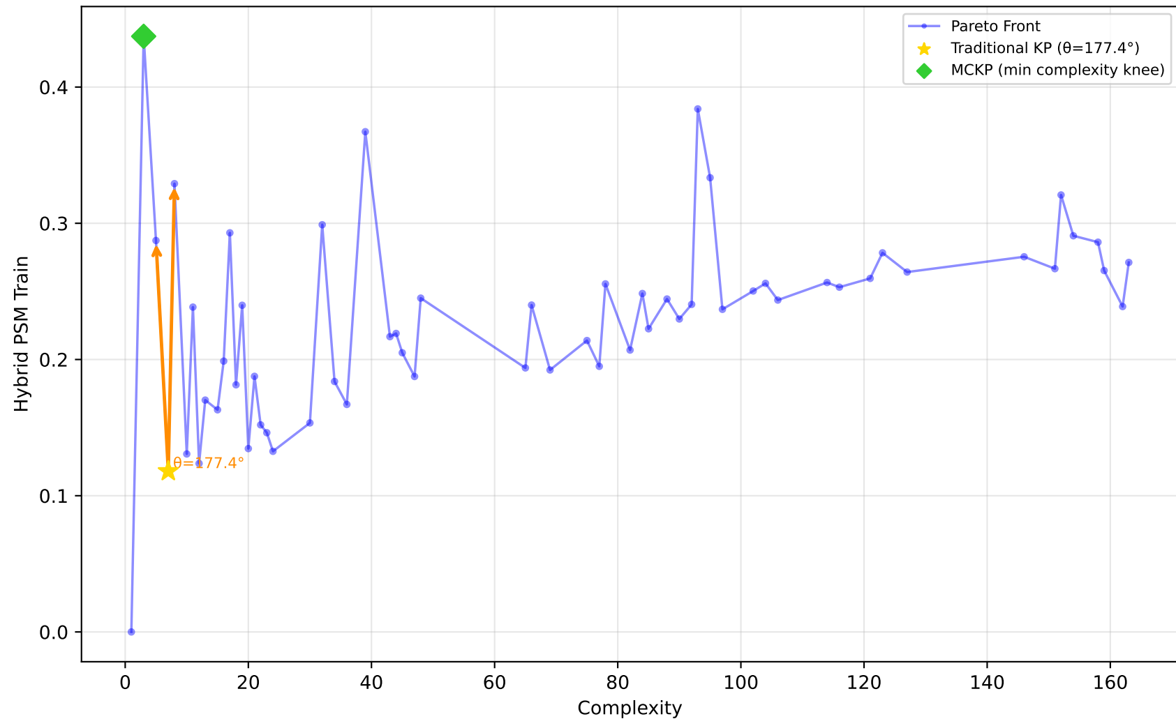
192_vineyard - Run 9 - SVP - Hybrid PSM Train \lambda_1=0.70, \lambda_2=0.70, \lambda_3=0.90 | Difficulty: 1.00 | Method: hmr
