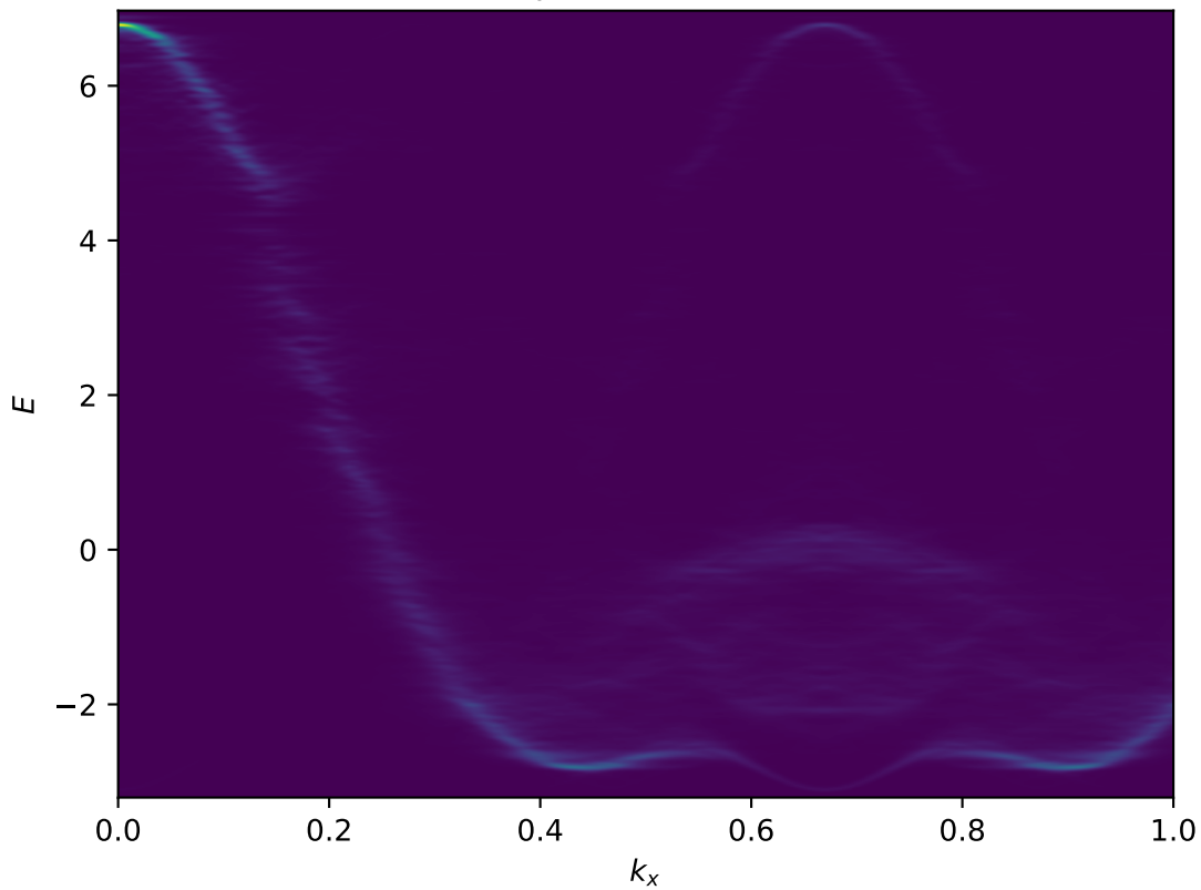
Dispersion relation
