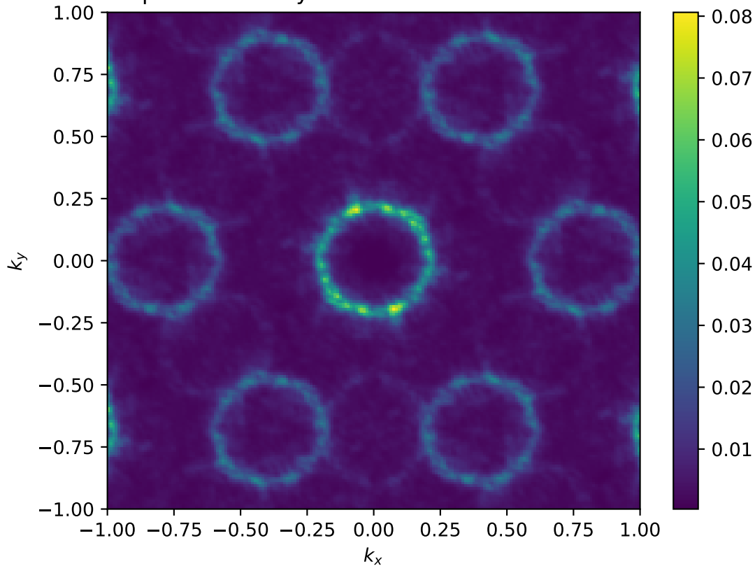
Spectral density at E = 6.737859132674986
