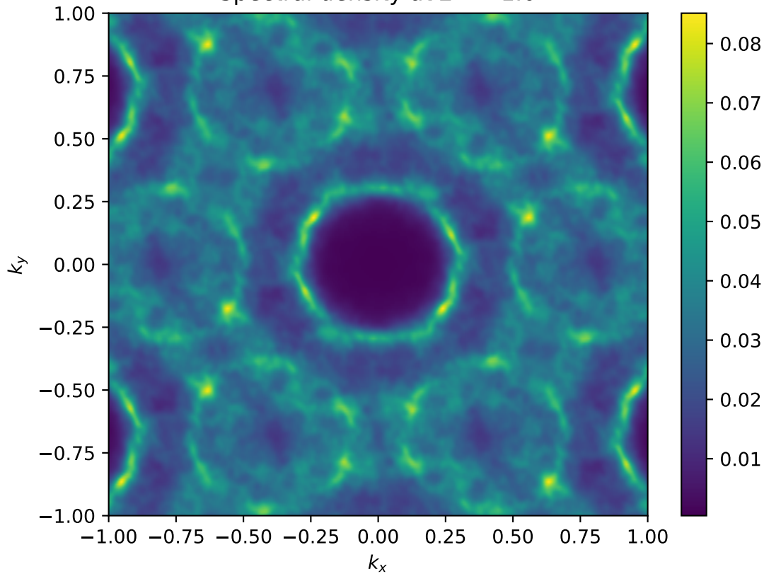
Spectral density at E = -1.0
