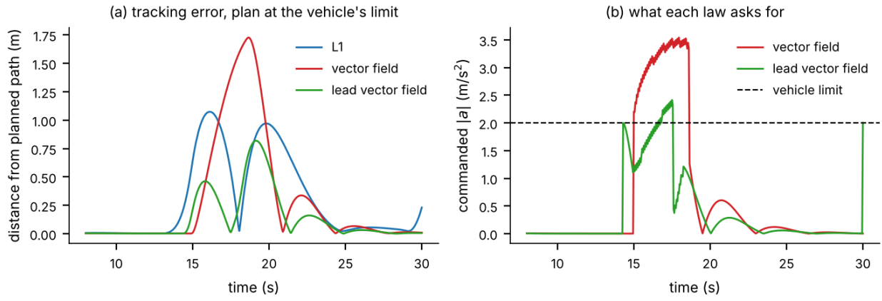
Figure 2. Quadcopter model, no wind, plan at the limit, one route. (a) Distance from the planned path. (b) Commanded sideways acceleration against the vehicle limit.
