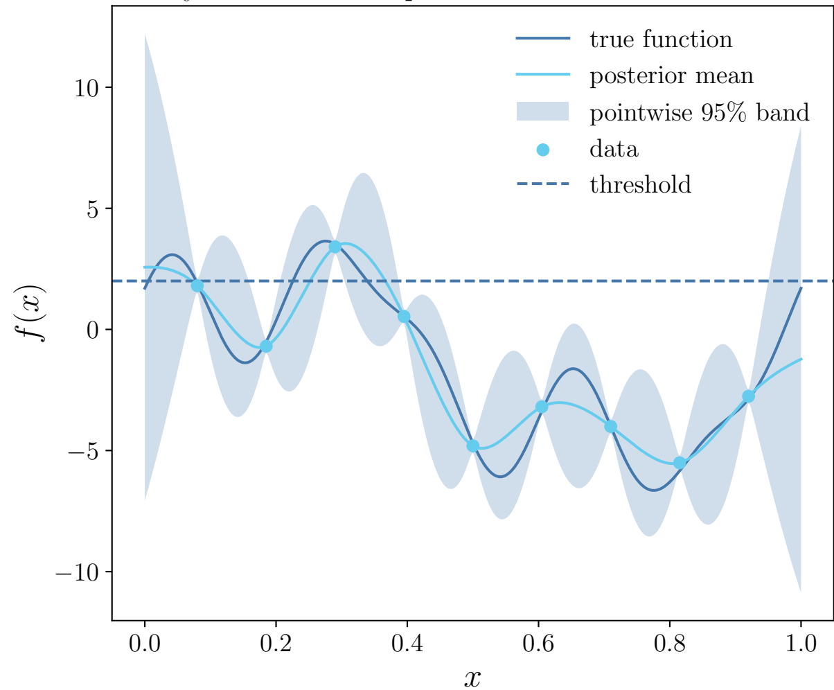
Bayesian Gaussian posterior for a latent function
