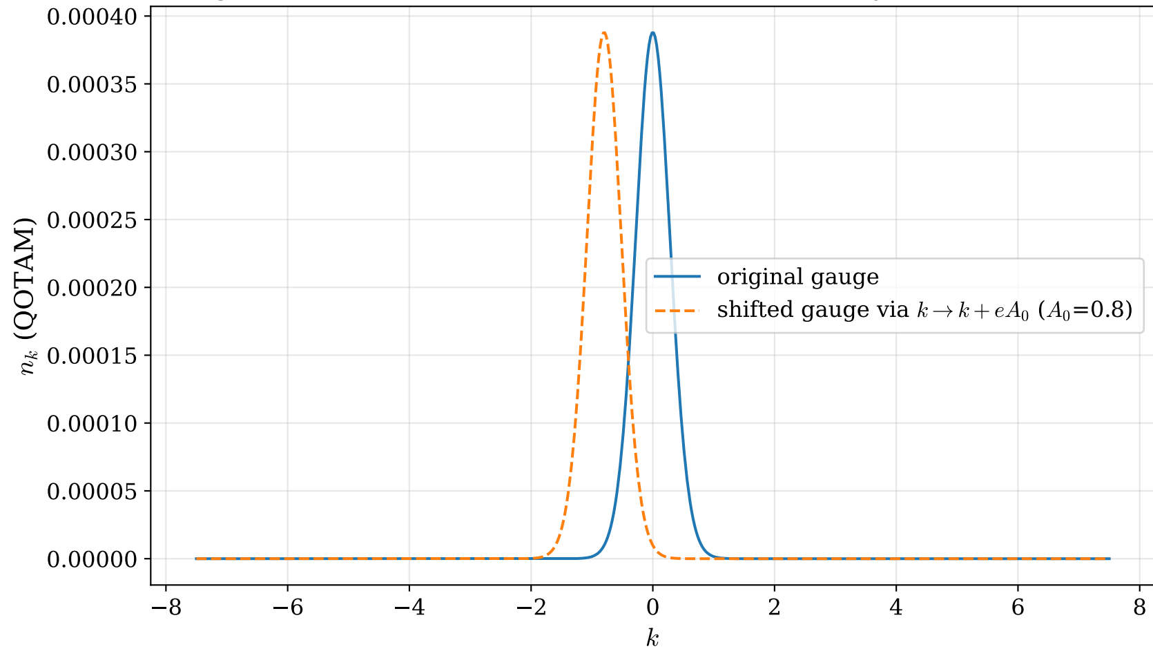
Gauge-equivalence (QOTAM): spectrum consistency ( E_0=0.300 , \tau=2.5 )
