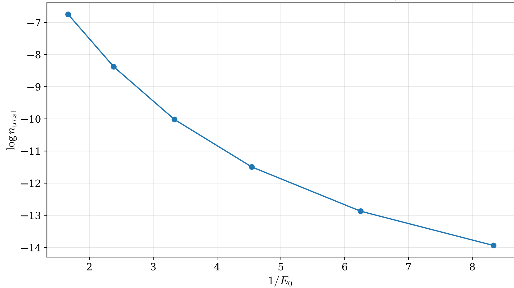
QOTAM non-perturbative scaling: \log(n_{total}) vs 1/E_0 ( \tau=2.5 )
