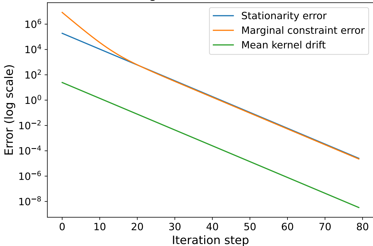
Convergence behavior of QOTAM
