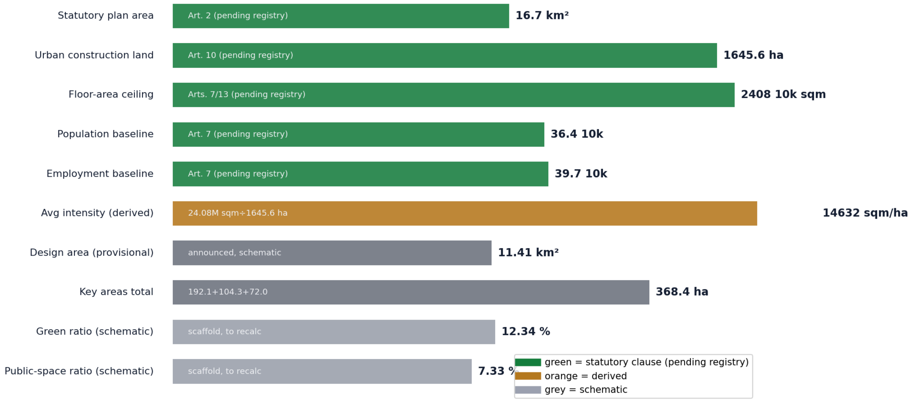
Fig. 5 Core Metrics Recalculation & Confidence Grading
