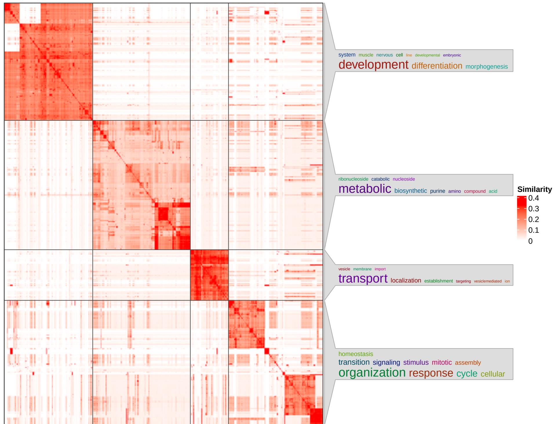
2045 GO terms clustered by 'binary_cut'
