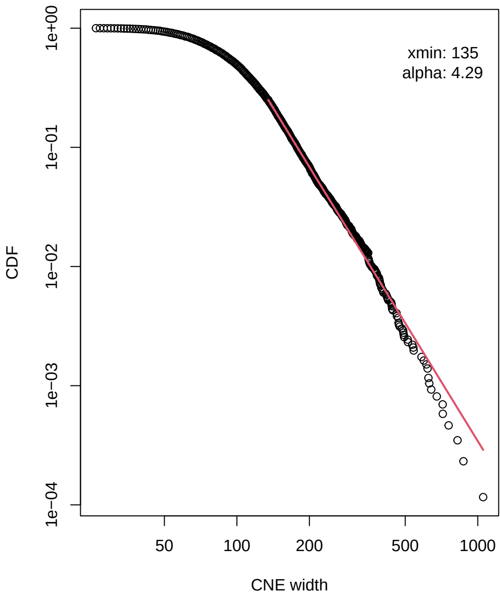
Power-law like distribution of Actinopteriigly specific CNE widths
