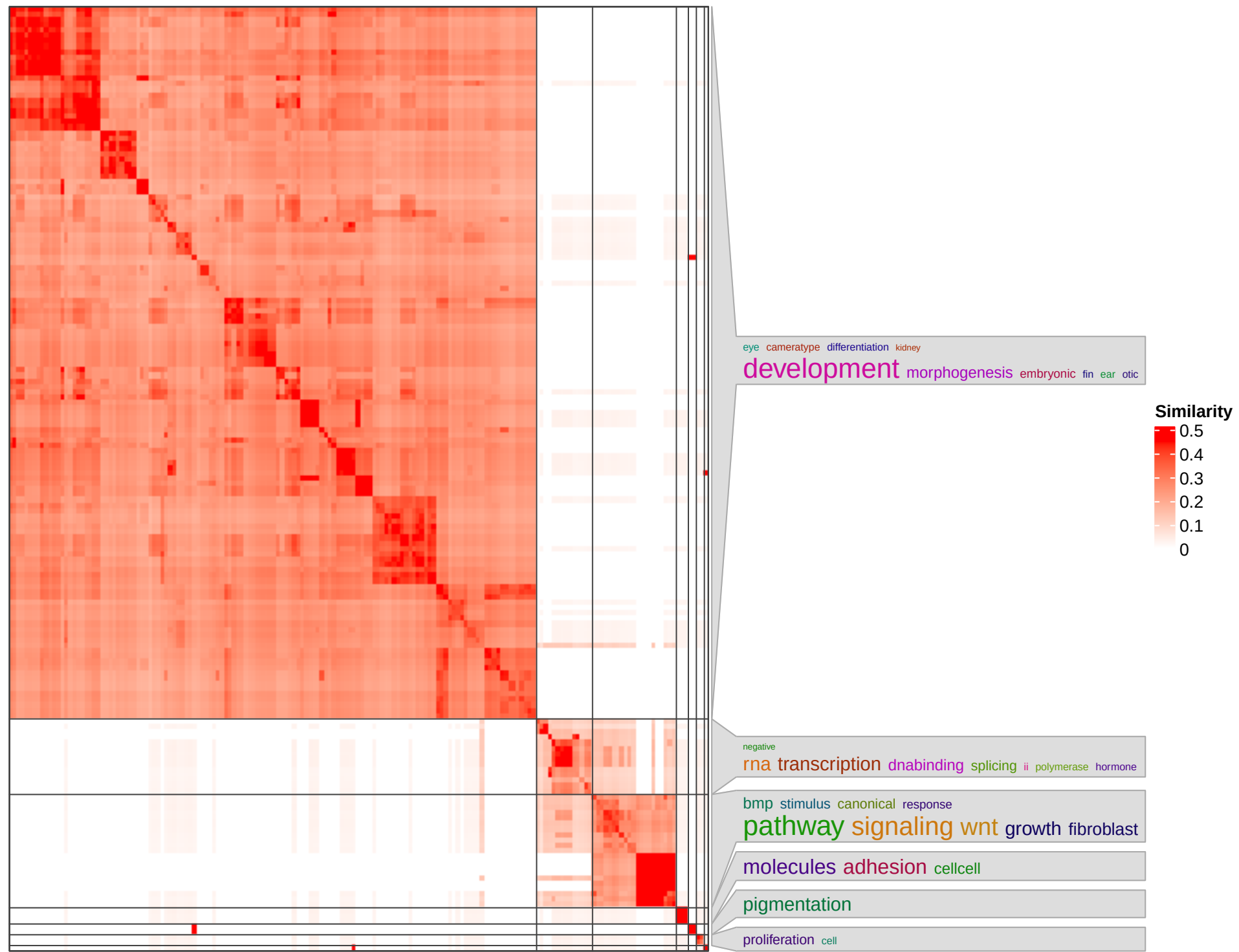
175 GO terms clustered by 'binary_cut'
