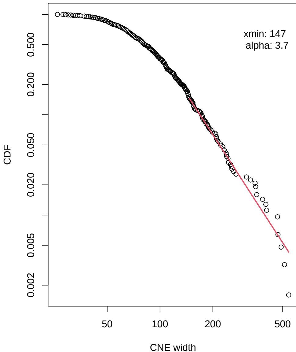
Power-law like distribution of Actinopteriig specific CNE widths
