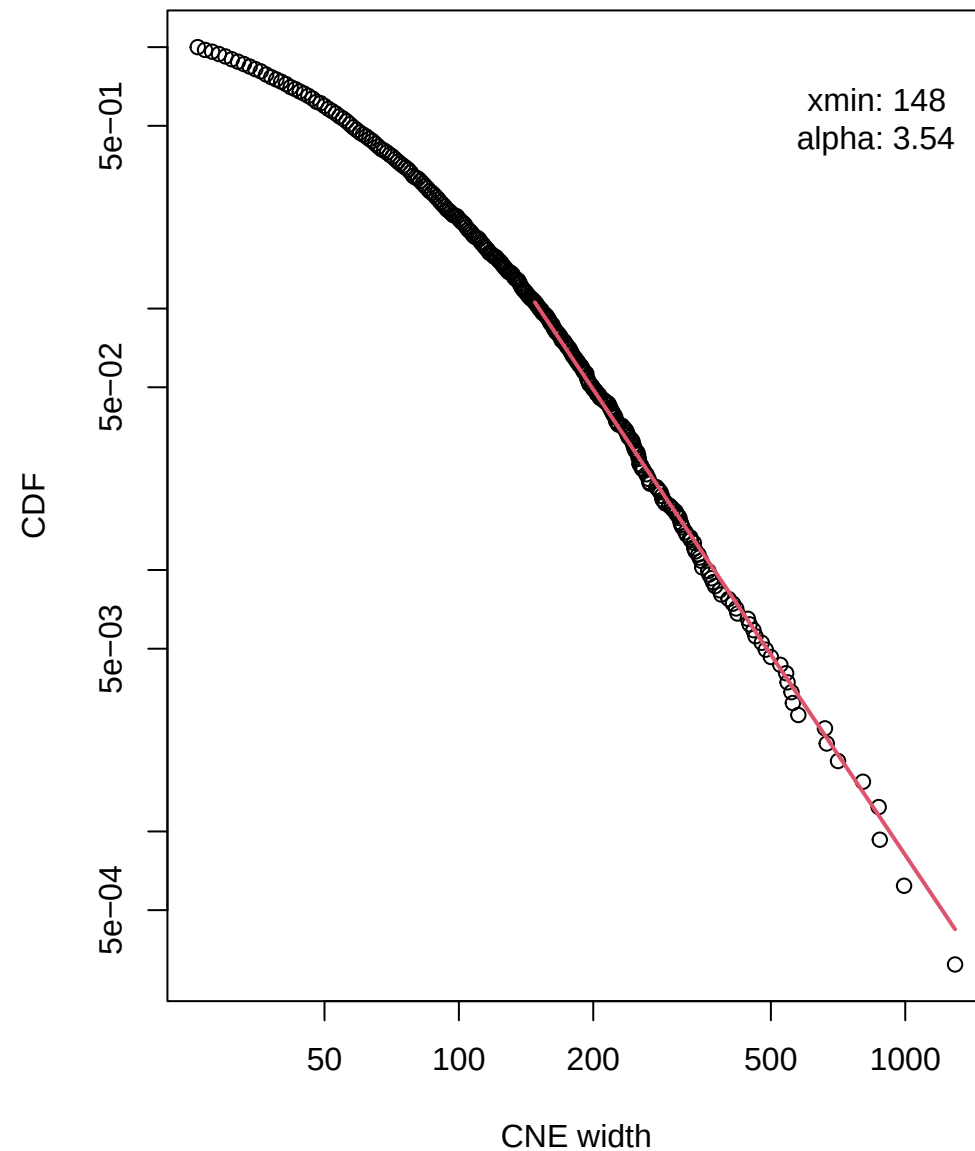
Power-law like distribution of Gnathostomata specific CNE widths
