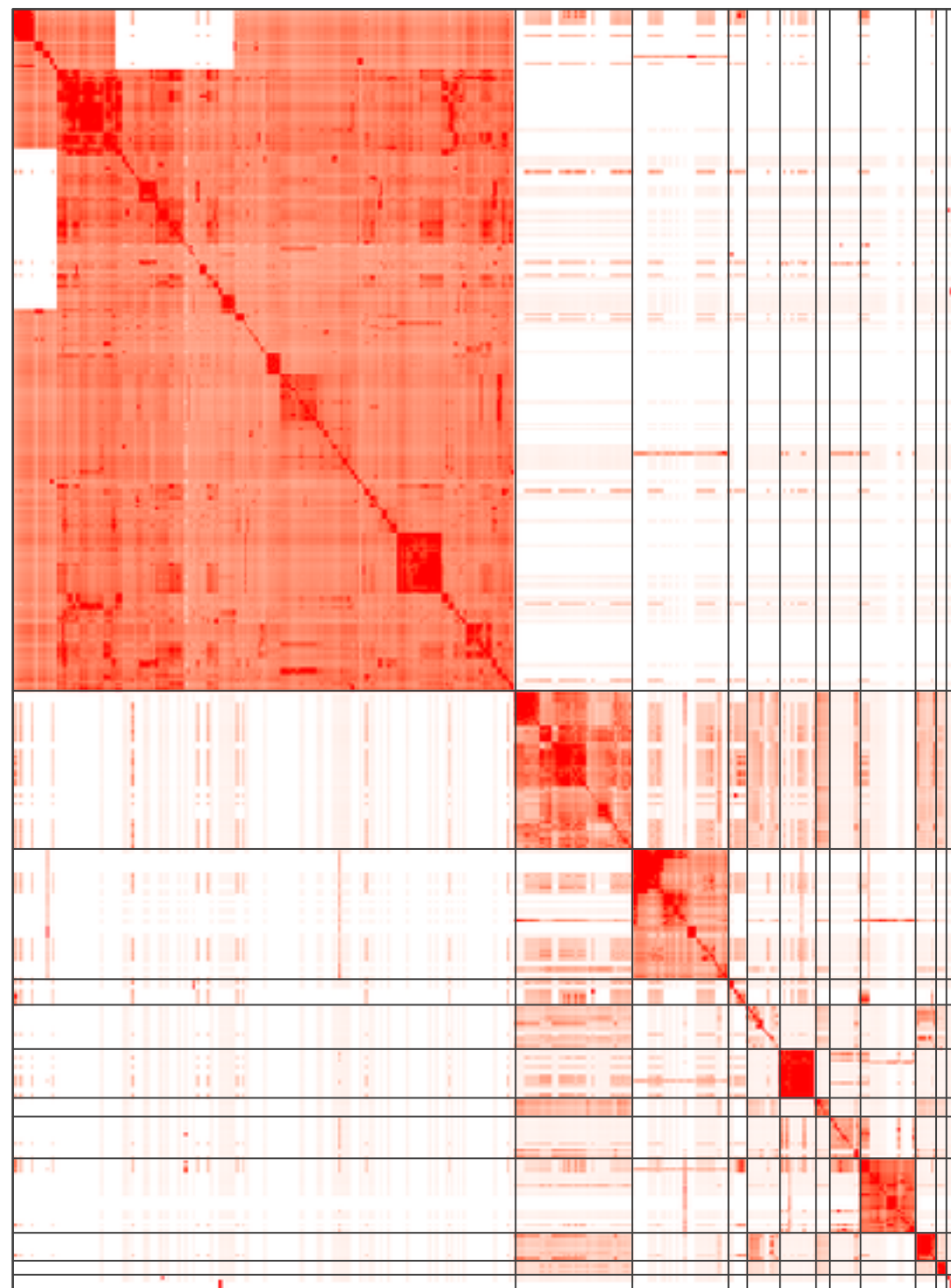
551 GO terms clustered by 'binary_cut'
