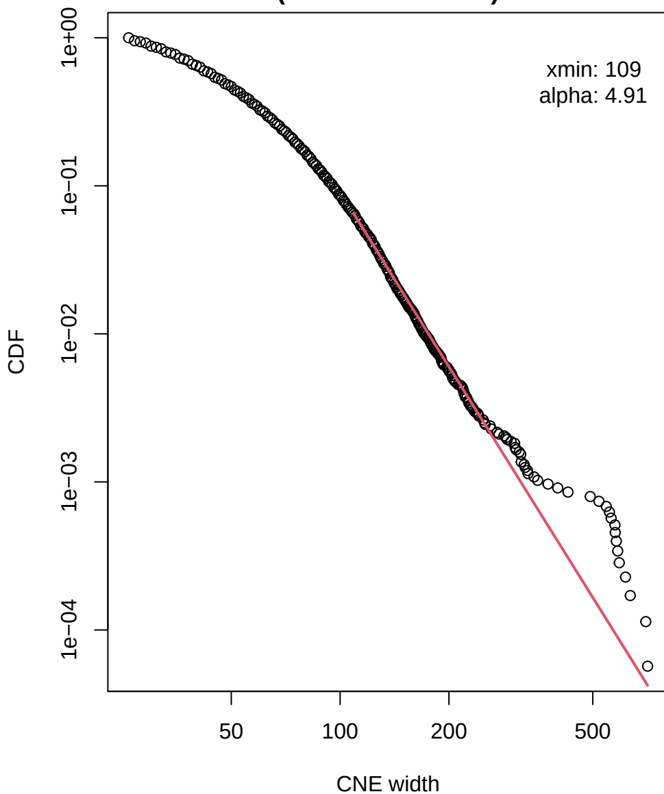
Power-law like distribution of Gnathostomata conserved CNE widths (human reference)
