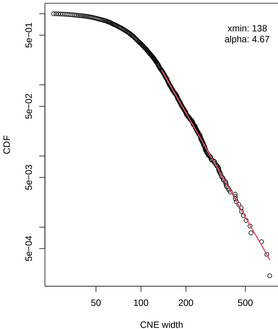
Power-law like distribution of Sarcopterygii specific CNE widths
